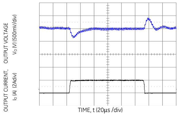
Figure 40. Transient Response to Dynamic Load Change from 0% 50% to 0%.
