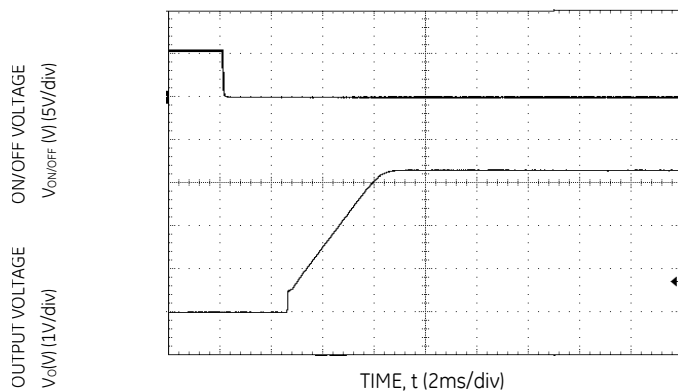
Figure 29. Typical Start-up Using On/Off Voltage (Io = Io,max).
