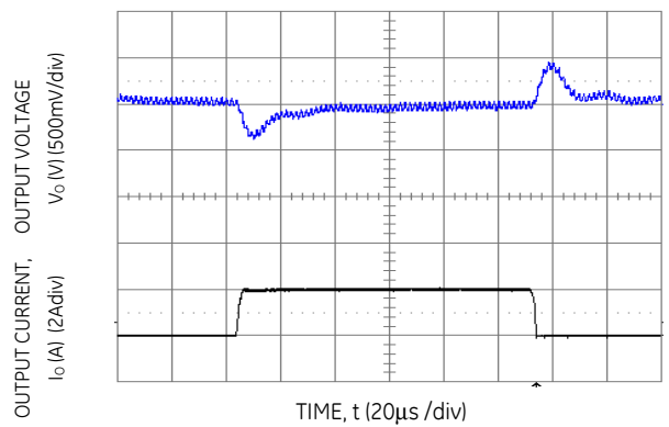
Figure 46. Transient Response to Dynamic Load Change from 0% 50% to 0%.
