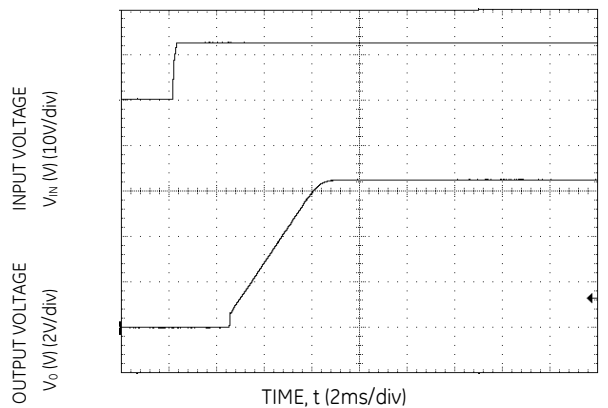
Figure 42. Typical Start-up Using Input Voltage ( V_{IN} = 12V , I_o = I_{o,max} ).
