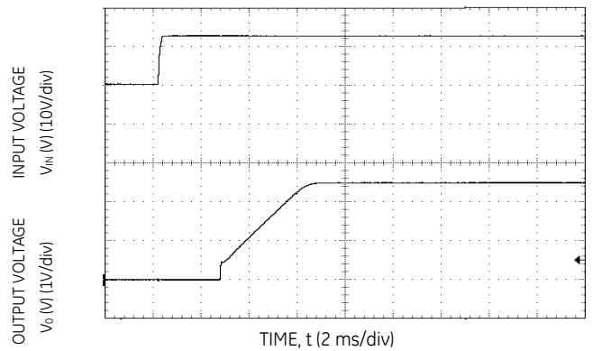
Figure 24. Typical Start-up Using Input Voltage ( V_{IN} = 12V , I_o = I_{o,max} ).
