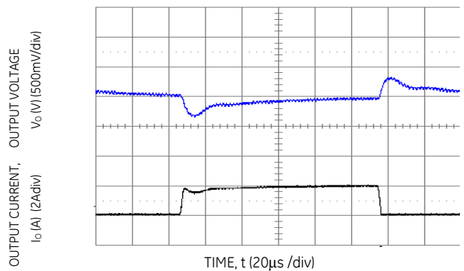
Figure 10. Transient Response to Dynamic Load Change from 0% to 50% to 0%.
