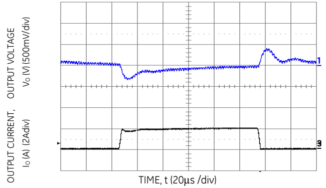
Figure 16. Transient Response to Dynamic Load Change from 0% to 50% to 0%.
