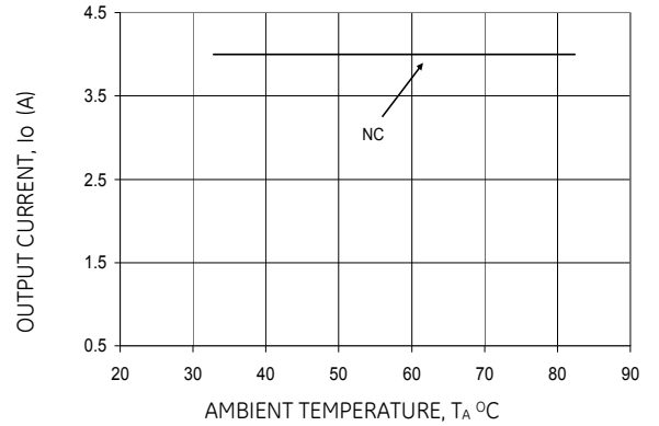
Figure 44. Derating Output Current versus Ambient Temperature and Airflow.
