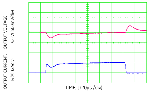
Figure 4. Transient Response to Dynamic Load Change from 0% to 50% to 0% .
