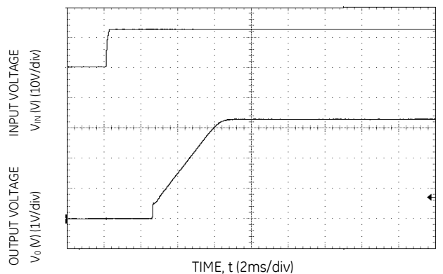
Figure 30. Typical Start-up Using Input Voltage (VIN = 12V, Io = Io,max).
