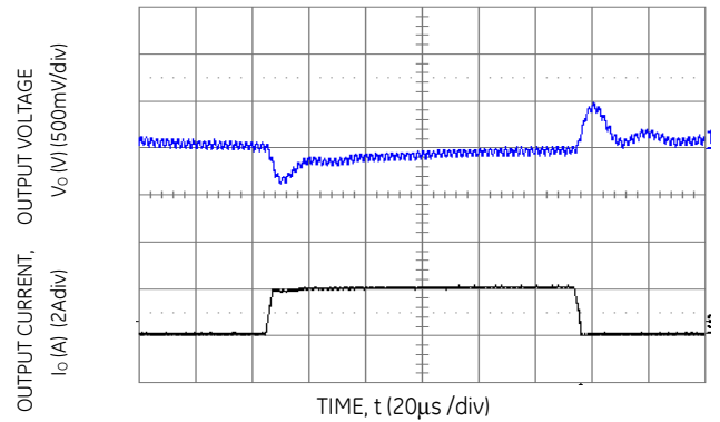
Figure 28. Transient Response to Dynamic Load Change from 0% 50% to 0%.
