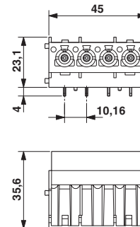
Dimensional drawing
