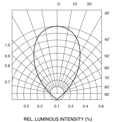
Fig. 4 Radiation Diagram
