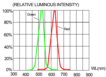
FIG.5 RELATIVE LUMINOUS INTENSITY VS. WAVELENGTH.
