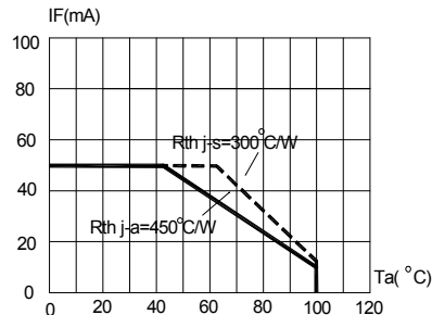
FIG.4a RED MAXIMUM FORWARD DC CURRENT VS AMBIENT TEMPERATURE ( T_{jmax}=110^{\circ}C )
