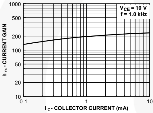
Figure 21. Current Gain
