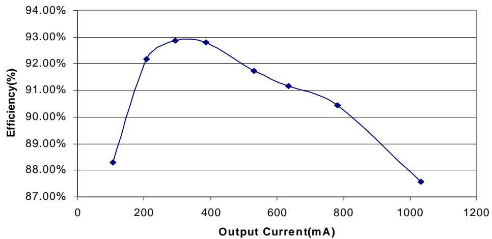
Figure 6 - Efficiency
