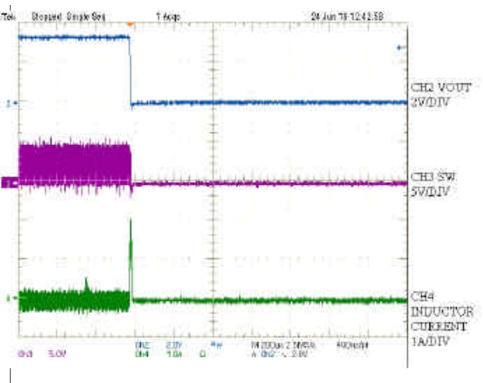
Figure 10 - Output short
