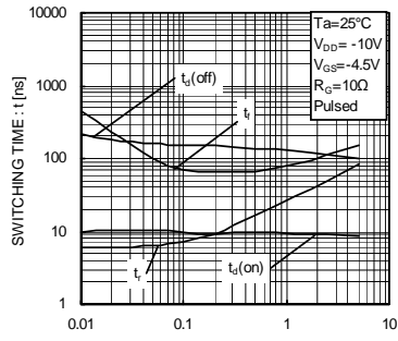
Fig.14 Switching Characteristics
