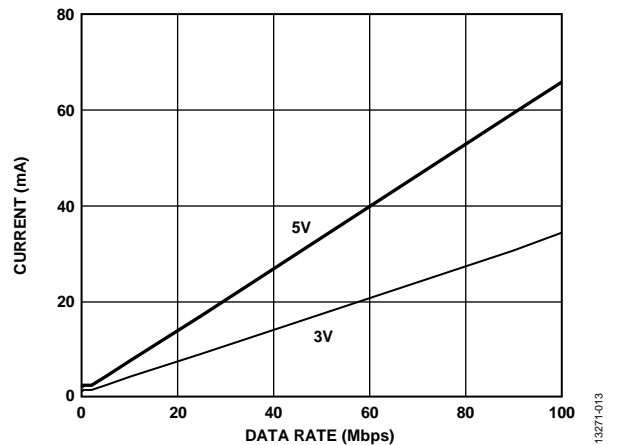
Figure 13. Typical ADuM3401-EP V_{DD1} Supply Current vs. Data Rate for 5V and 3.3V Operation
