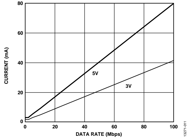
Figure 11. Typical ADuM3400-EP V_{DD1} Supply Current vs. Data Rate for 5V and 3.3V Operation
