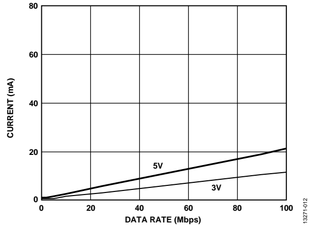
Figure 12. Typical ADuM3400-EP V_{DD2} Supply Current vs. Data Rate for 5V and 3.3V Operation
