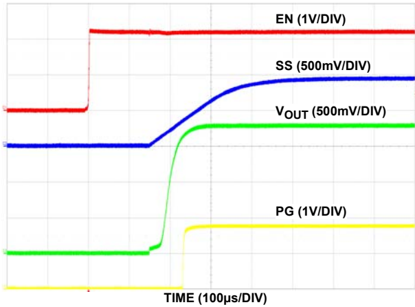
FIGURE 15. ENABLE START-UP SS CAP 1nF
