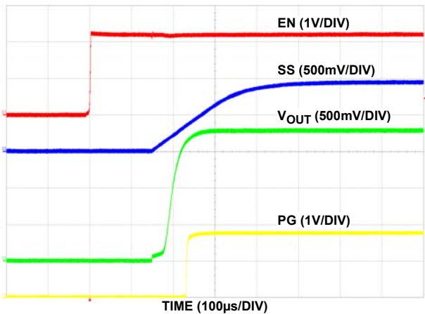
FIGURE 17. ENABLE START-UP SS CAP 100nF
