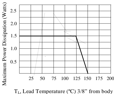
Figure 1. Power Derating Curve
