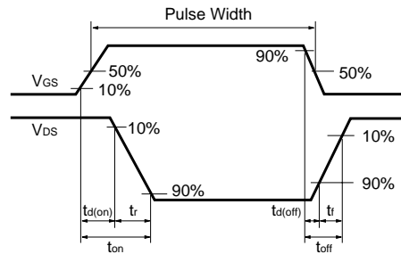
Fig.14 Switching Waveforms
