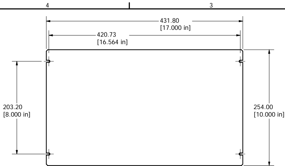
1434-30 - VIEW FROM TOP (SOLD SEPERATELY)
