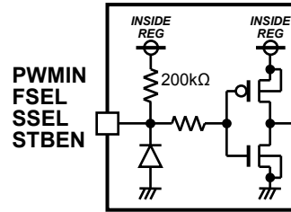
2. PWM signal input Drive PWM frequency select FG/AL signal select Standby mode enable select
