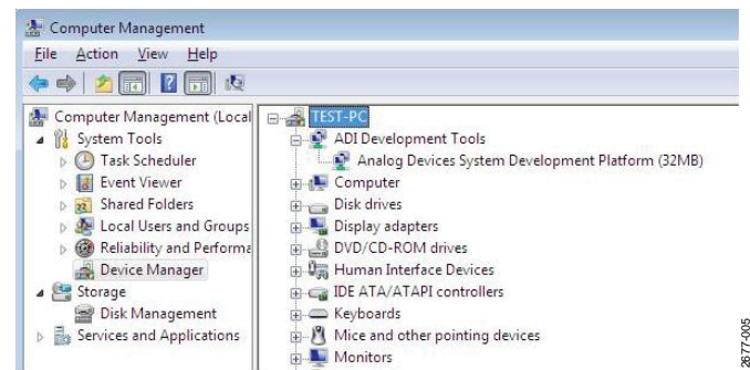
Figure 5. Device Manager
