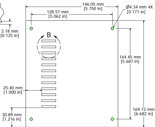
ENCLOSURE CASE - BOTTOM VIEW
