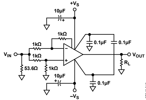
Figure 52. Common-Mode Rejection
