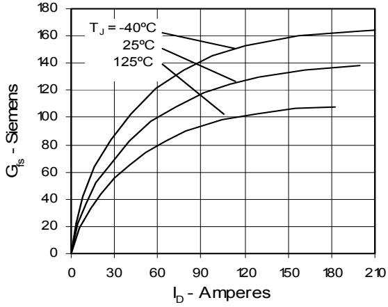
Fig. 7. Transconductance
