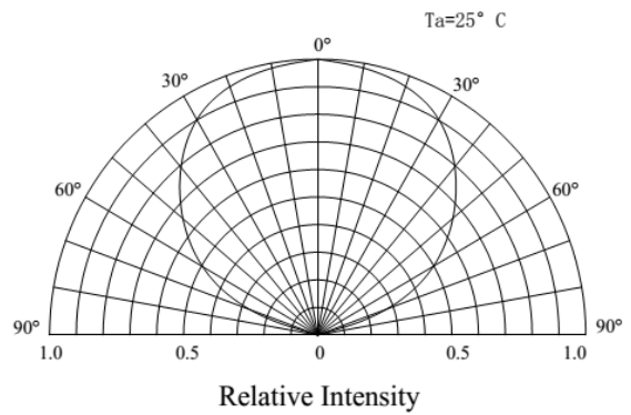
RADIATION PATTERN
