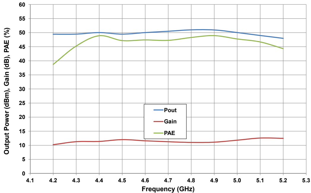
Figure 2. - Modulated @ Spectral Regrowth = -30dBc, 1.6 MHz from Carrier 1.6 Msps OQPSK Modulation V_{DD} = 40\text{ V} , I_{DQ} = 1\text{ A} , T_{case} = 25^\circ\text{C}
