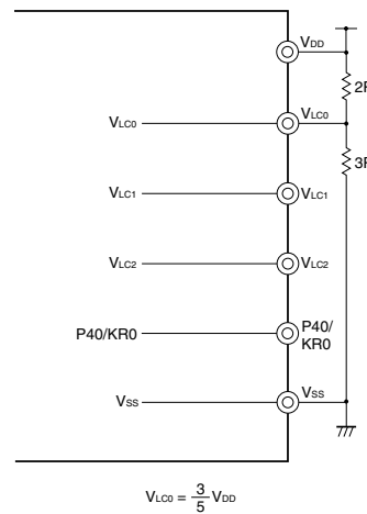
(b) Static display mode (MDSET1, MDSET0 = 0, 0) (example of V_{DD} = 5\text{ V} , V_{LC0} = 3\text{ V} )
