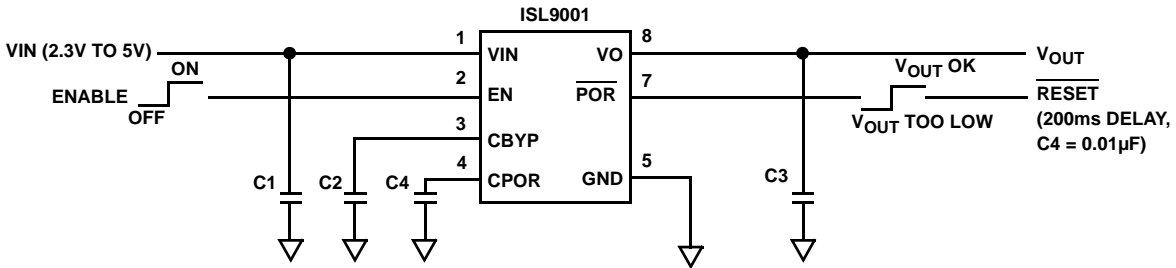
C1, C3: 1 \mu F X5R CERAMIC CAPACITOR C2: 0.1 \mu F X7R CERAMIC CAPACITOR C4: 0.01 \mu F X7R CERAMIC CAPACITOR
