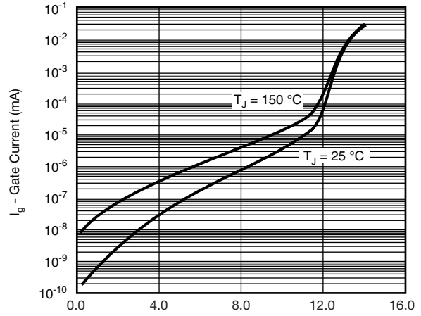
T_J = 150\text{ }^\circ\text{C} T_J = 25\text{ }^\circ\text{C} Gate Current vs. Gate-Source Voltage
