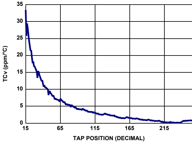
FIGURE 17. 100k TCv vs TAP POSITION
