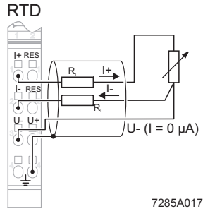
Figure 20 RTD 3-wire connection
