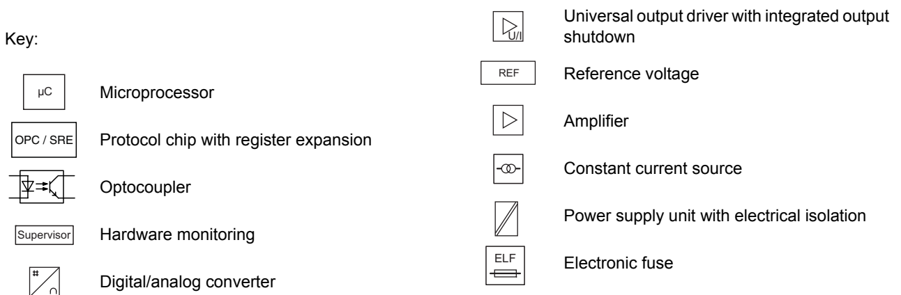
Figure 2 Internal wiring of the terminal points
