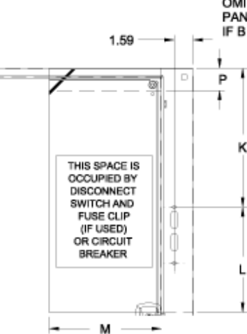
Disconnect Mounting Details
