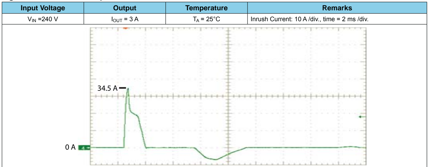
Figure 5. Inrush Current Operation
