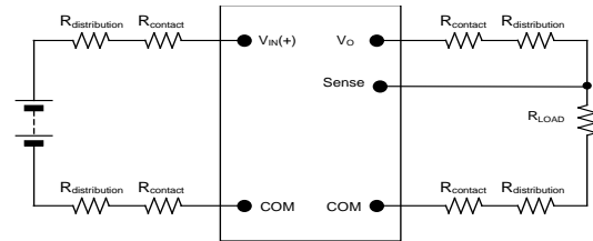
Figure 33. Remote sense circuit configuration.
