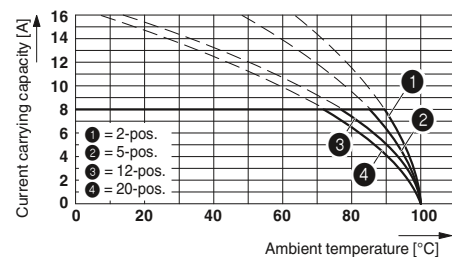
Type: MC 1,5/...-ST-3.81 with SMC 1,5/...-G-3.81
