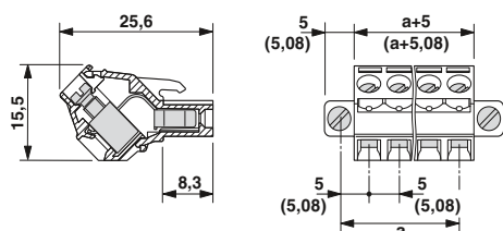
Type: SMSTB 2,5/...-ST with MSTBA 2,5/...-G
