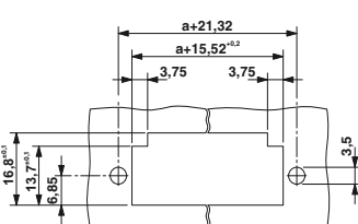
For screw fixing
