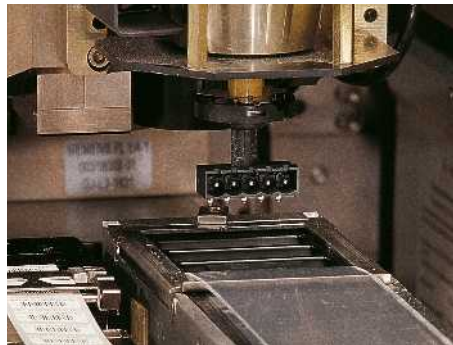
Component picked from the tape
