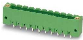
With threaded flange, plug-in direction vertical to the PCB
