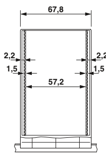
Housing inner dimensions
