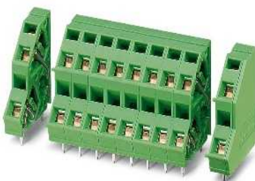
Double-level PCB terminal block, compact design, without actuation rocker
