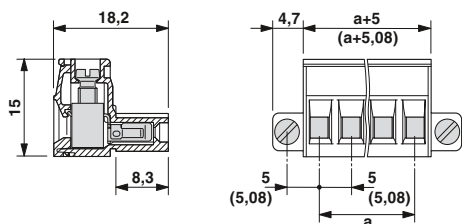
Type: MSTB 2,5 HC/...-ST with MSTBA 2,5 HC/...G
