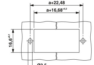
For screw fixing
