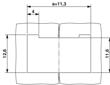
DMCV 1,5/...-G1F-3,5-LR P20THR, see page 187.
