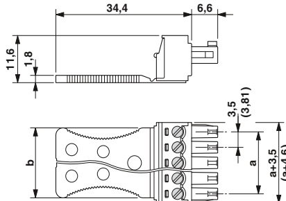
Type: MC 1,5/...-ST-3.81 with MC 1,5/...-G-3.81
