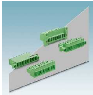
PC 4 series: feed-through plug screw or solder connection, up to 20 A, 7.62 mm pitch DFK-PC 4... Page 518
