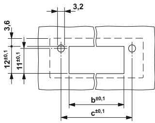
Sheet metal cutouts for DFK-MSTB 2,5/...-G, see page 352.
