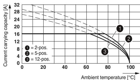
Type: MSTB 2,5 HC/...-ST with MSTBA 2,5 HC/...G
