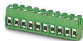
Plugs with screw connection, can be horizontally and vertically plugged onto PST 1,3/...-5,0 pin strips
