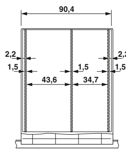
Housing inner dimensions
