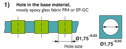
Structure of the metal-plated hole for EMSTB(A) 2,5/...-G(F)-... and EMSTBV(A) 2,5/...-G(F)-...
