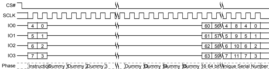
Figure 8.8 Read Unique ID (RUID) QPI Mode Command
