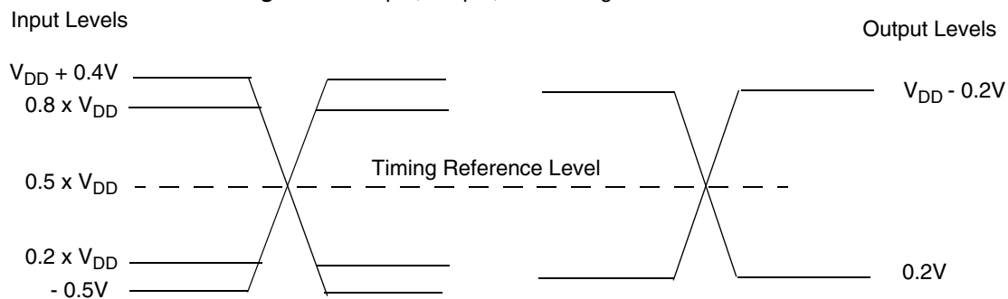
Figure 12.3 Input, Output, and Timing Reference Levels
