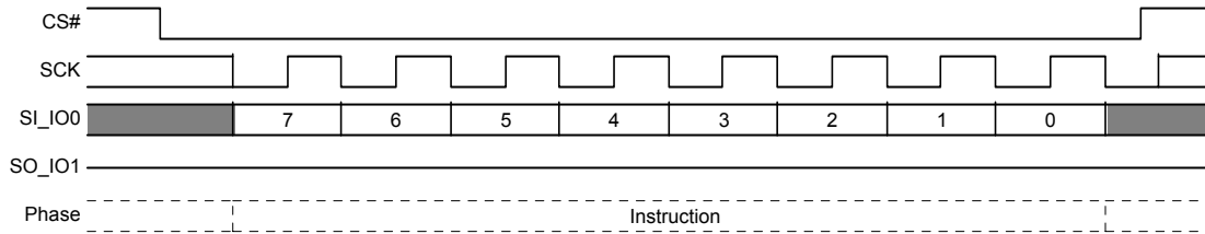
Figure 8.60 Chip Erase Command Sequence
