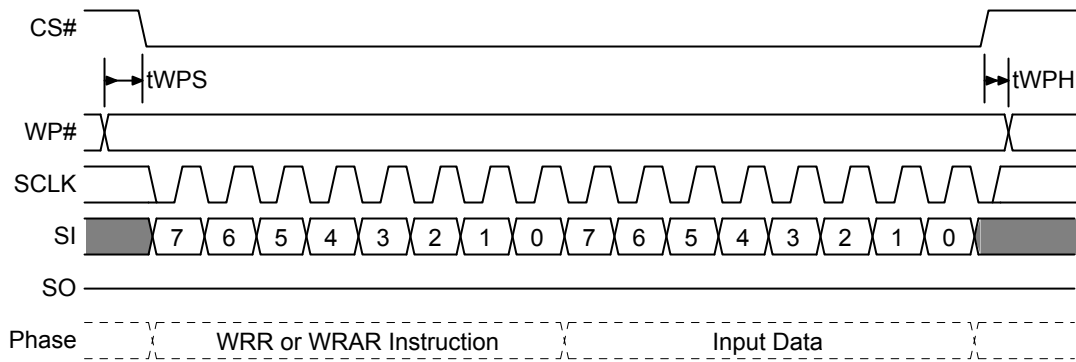
Figure 12.14 WP# Input Timing
