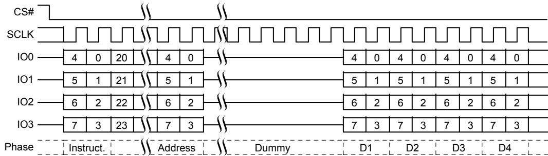
Figure 8.6 RSFDP QPI Mode Command Sequence
