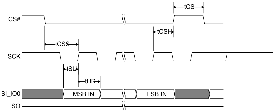
Figure 12.11 SPI Single Bit Input Timing
