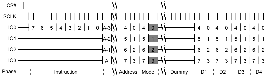
Figure 8.45 Quad I/O Read Initial Access Command Sequence
