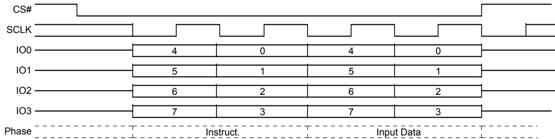
Figure 8.24 Program DLRNV (PDLRNV) Command Sequence – QPI Mode
