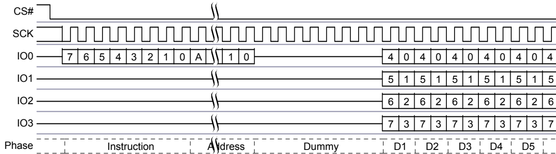
Figure 8.42 Quad Output Read Command Sequence
