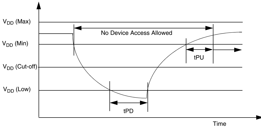
Figure 11.4 Power-down and Voltage Drop
