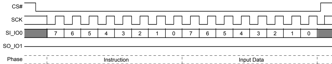
Figure 8.23 Program DLRNV (PDLRNV) Command Sequence
