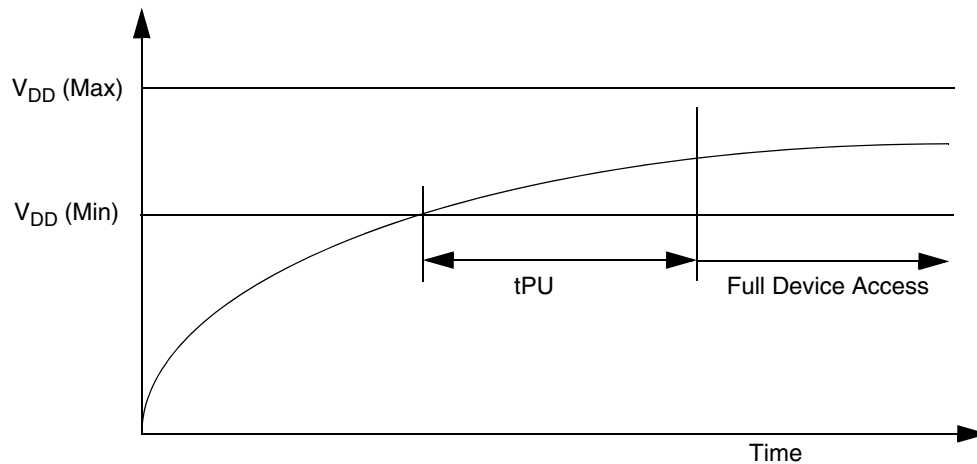
Figure 11.3 Power-up
