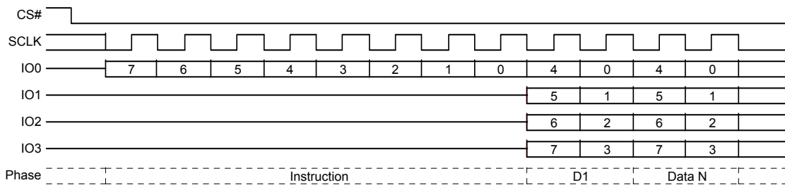
Figure 8.4 Read Quad Identification (RDQID) Command Sequence Quad Mode
