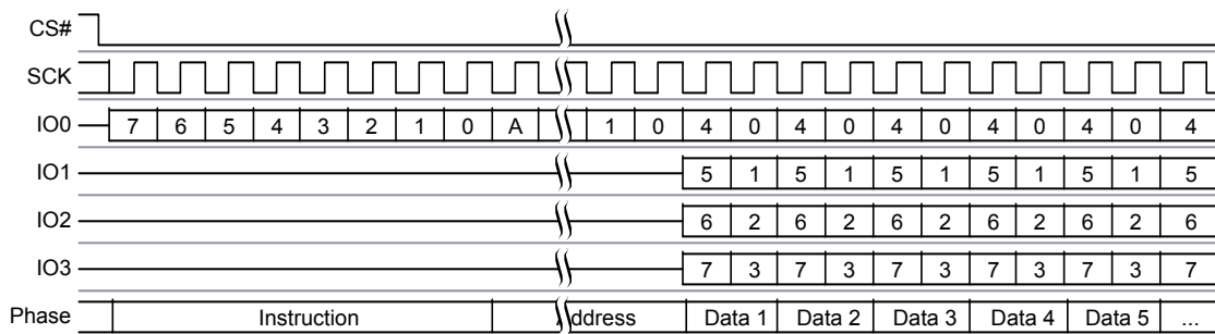
Figure 8.53 Quad Page Program Command Sequence
