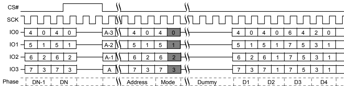
Figure 8.47 Continuous Quad I/O Read Command Sequence
