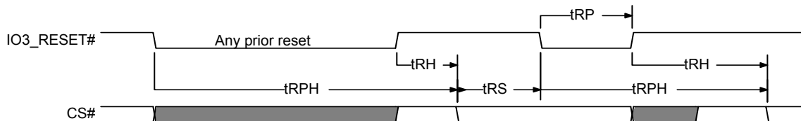
Figure 12.8 Hardware Reset when Quad or QPI Mode is not enabled and IO3 / RESET# is Enabled
