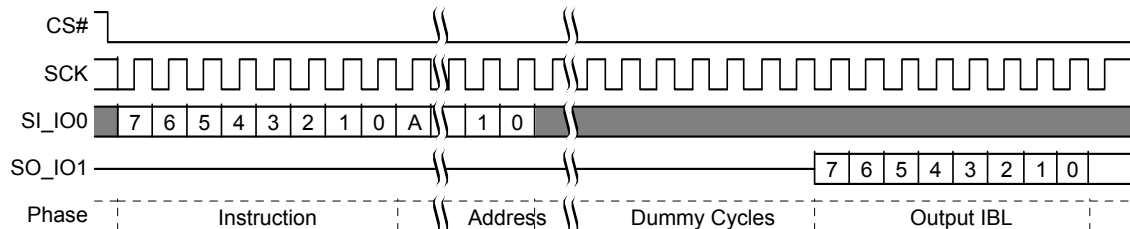
Figure 8.69 IBLRD Command Sequence
