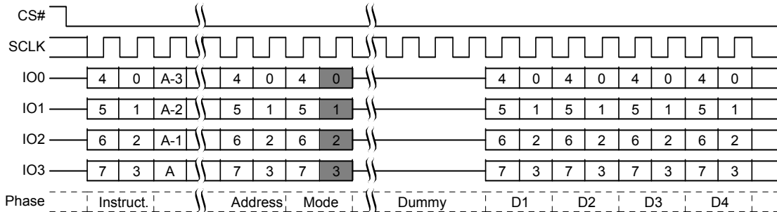
Figure 8.46 Quad I/O Read Initial Access Command Sequence QPI mode
