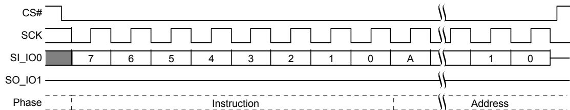
Figure 8.71 IBL Command Sequence
