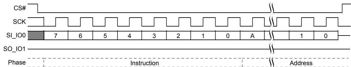
Figure 8.54 Sector Erase (SE 20h or 4SE 21h) Command Sequence
