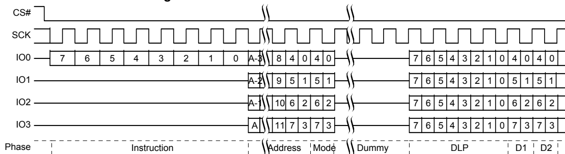
Figure 8.48 DDR Quad I/O Read Initial Access
