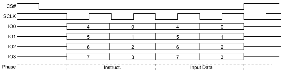
Figure 8.26 Write DLRV (WDLRV) Command Sequence – QPI Mode
