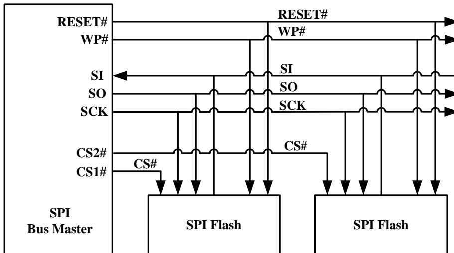
Figure 4.1 Bus Master and Memory Devices on the SPI Bus - Single Bit Data Path
