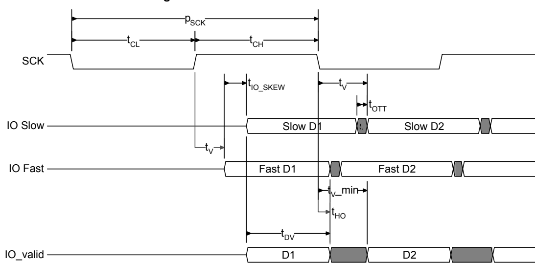
Figure 12.17 SPI DDR Data Valid Window
