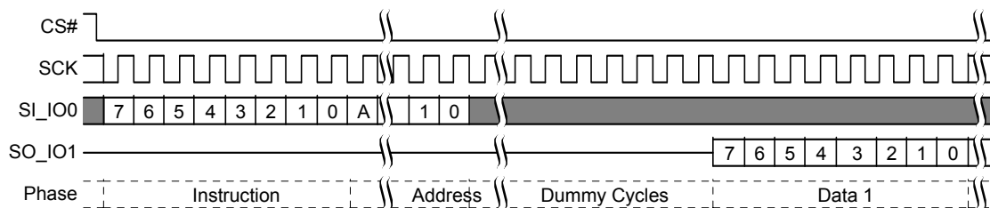
Figure 8.67 Security Regions Read Command Sequence
