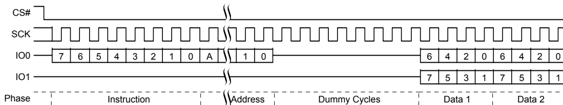
Figure 8.41 Dual Output Read Command Sequence
