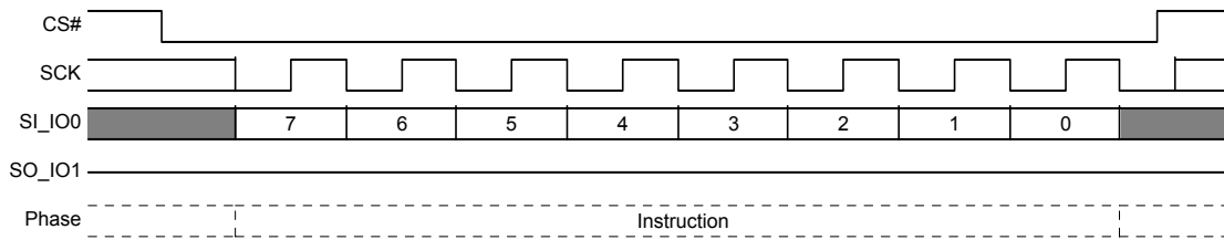
Figure 8.65 Erase or Program Resume command Sequence
