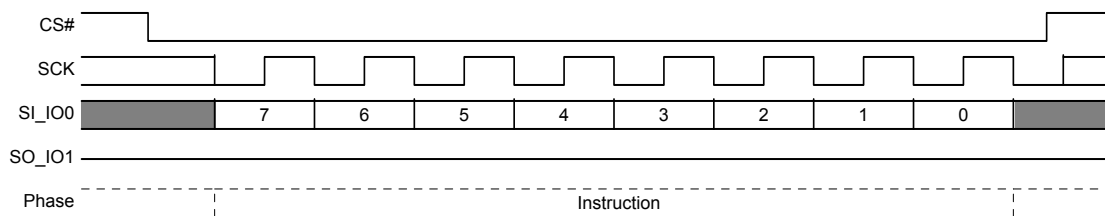
Figure 8.31 Exit 4 Byte Address Mode (4BEX E9h) Command Sequence
