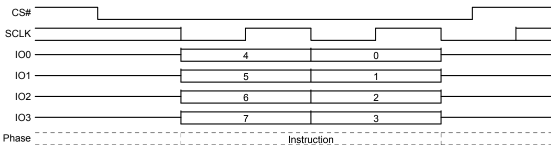
Figure 8.61 Chip Erase Command Sequence QPI Mode
