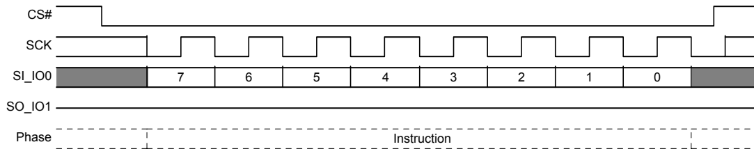
Figure 8.15 Write Enable (WREN) Command Sequence
