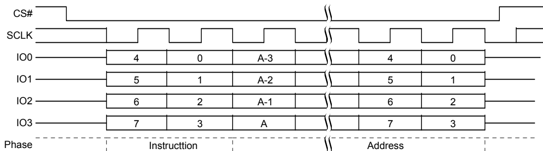
Figure 8.74 IBUL Command Sequence QPI Mode
