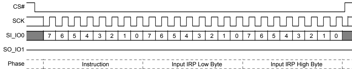
Figure 8.83 IRP Program (IRPP) Command
