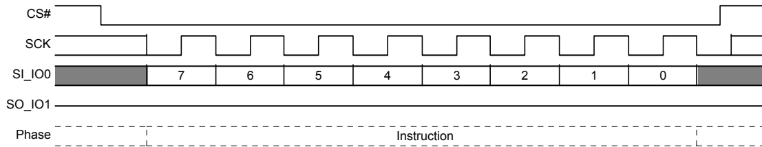
Figure 8.75 Global IBL Lock (GBL) Command Sequence
