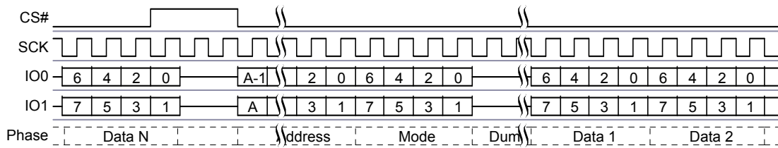
Figure 8.44 Dual I/O Continuous Read Command Sequence
