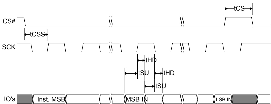
Figure 12.15 SPI DDR Input Timing
