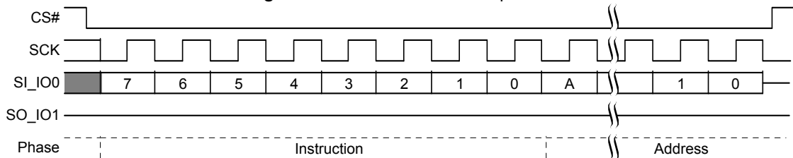
Figure 8.73 IBUL Command Sequence
