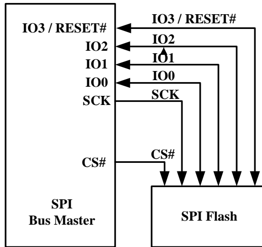
Figure 4.4 Bus Master and Memory Devices on the SPI Bus - Quad Bit Data Path - I/O3 / RESET#
