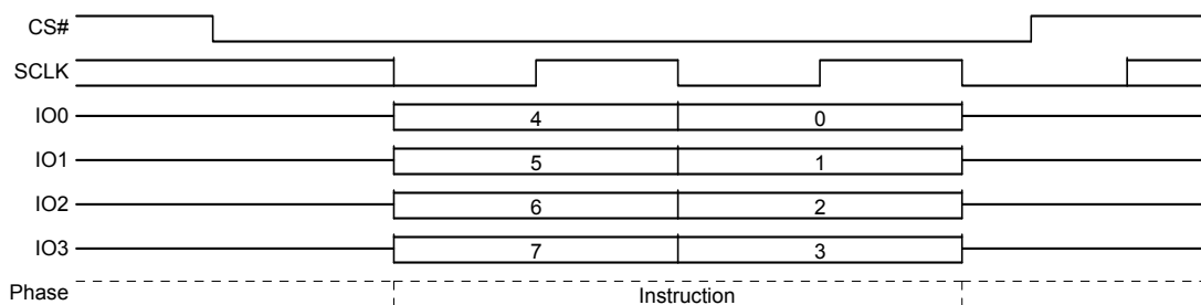
Figure 8.32 Exit 4 Byte Address QPI Mode
