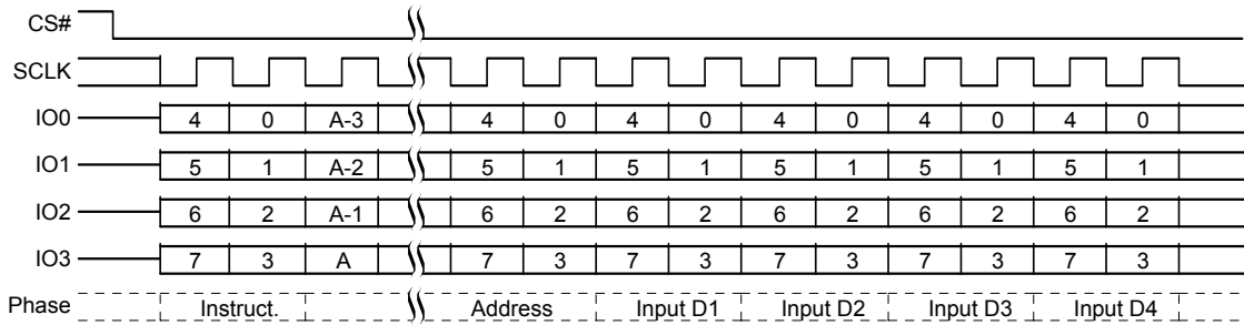
Figure 8.52 Page Program (PP 02h or 4PP 12h) QPI Mode Command Sequence
