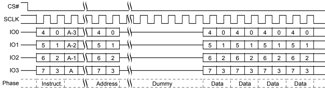
Figure 8.34 Read Any Register, QPI Mode, Command Sequence
