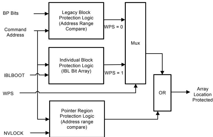
Figure 7.1 WPS Selection of LBP or IBL and PRP Array Protection
