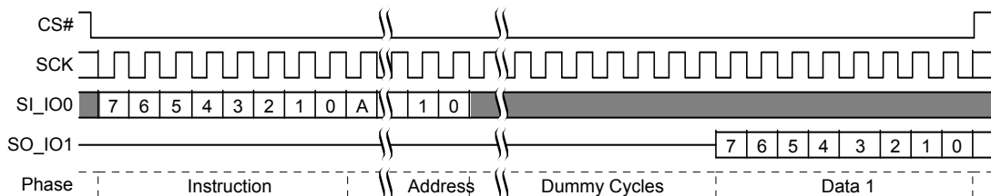
Figure 8.5 RSFDP Command Sequence
