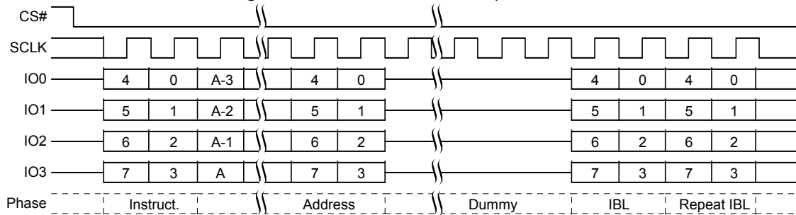
Figure 8.70 IBLRD Command Sequence QPI
