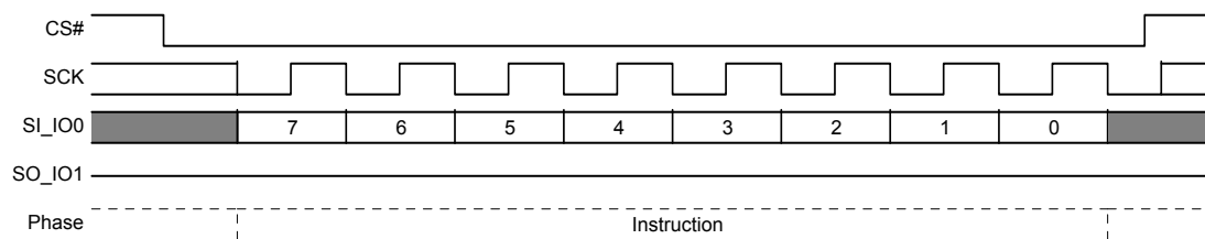
Figure 8.29 Enter 4 Byte Address Mode (4BEN B7h) Command Sequence
