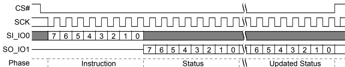
Figure 8.11 Read Status Register 1 (RDSR2) Command
