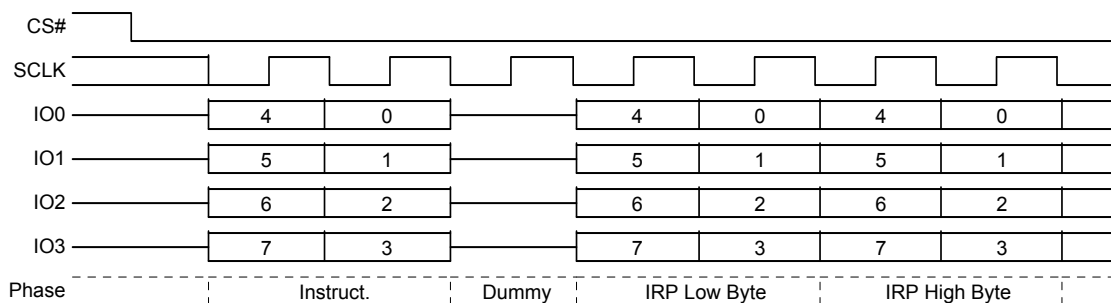
Figure 8.82 IRPRD Command Sequence – QPI Mode
