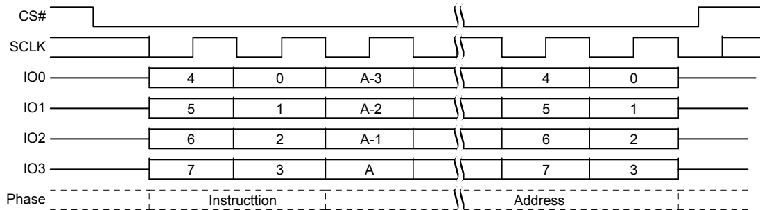
Figure 8.57 Half Block Erase (HBE 52h or 4HBE 53h) QPI Mode Command Sequence
