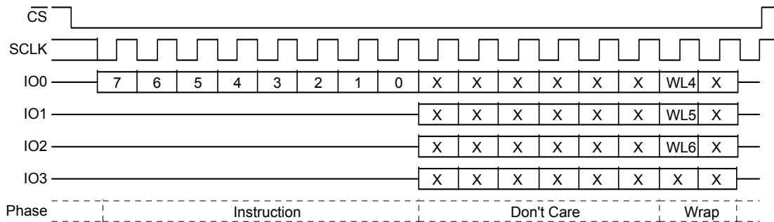
Figure 8.35 Set Burst Length Command Sequence Quad I/O Mode
