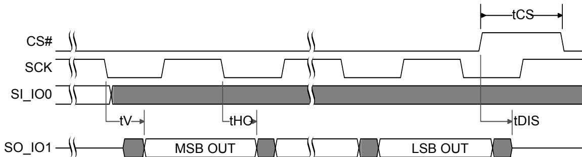
Figure 12.12 SPI Single Bit Output Timing
