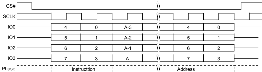
Figure 8.59 Block Erase (BE D8h or 4BE DCh) QPI Mode Command Sequence
