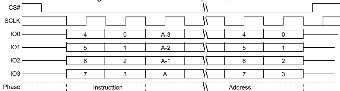
Figure 8.80 SPRP Command Sequence QPI Mode
