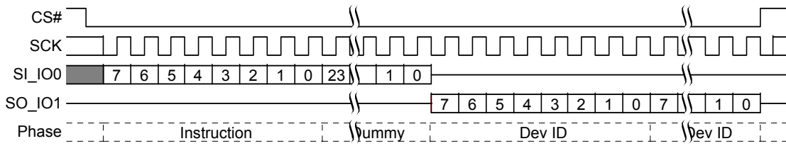
Figure 8.101 Read Identification (RES) Command Sequence
