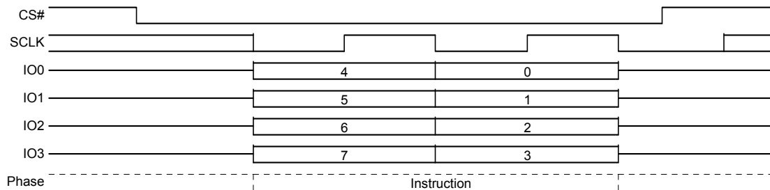
Figure 8.88 Protection Register Lock (PRL) Command Sequence – QPI Mode
