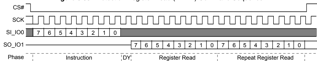
Figure 8.85 Protection Register Read (PRRD) Command Sequence
