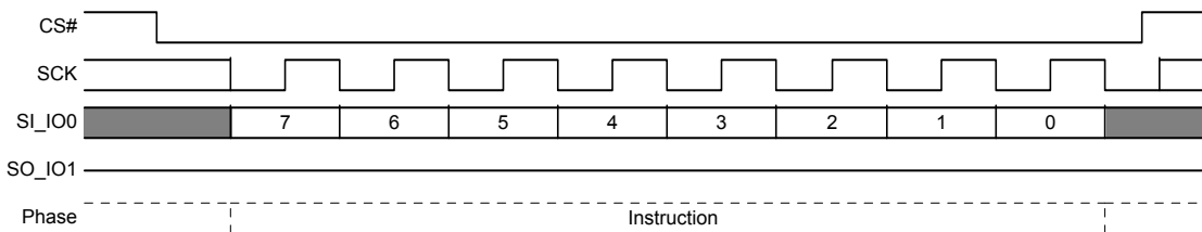
Figure 8.77 Global IBL Unlock (GBUL) Command Sequence
