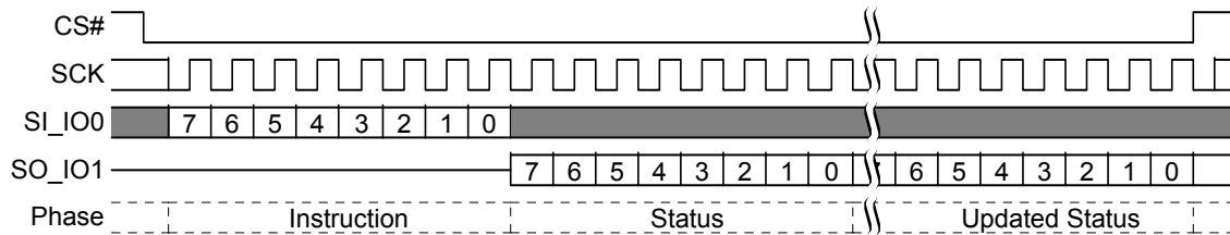
Figure 8.9 Read Status Register 1 (RDSR1) Command Sequence
