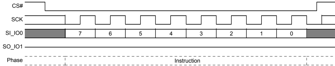
Figure 8.21 Clear Status Register (CLSR) Command Sequence
