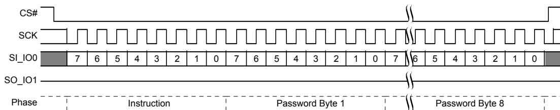
Figure 8.93 Password Unlock (PASSU) Command Sequence
