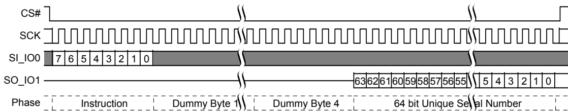
Figure 8.7 Read Unique ID (RUID) Command Sequence
