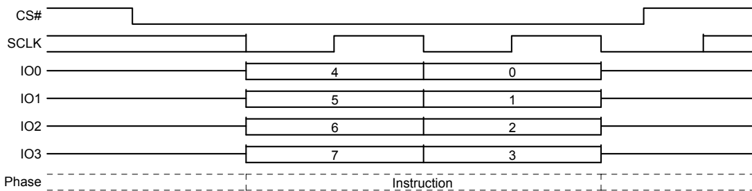
Figure 8.63 Program or Erase Suspend Command Sequence QPI mode
