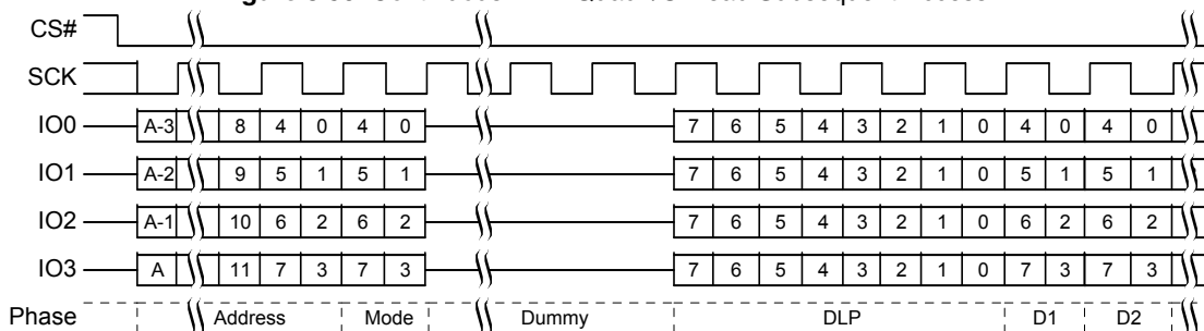
Figure 8.50 Continuous DDR Quad I/O Read Subsequent Access
