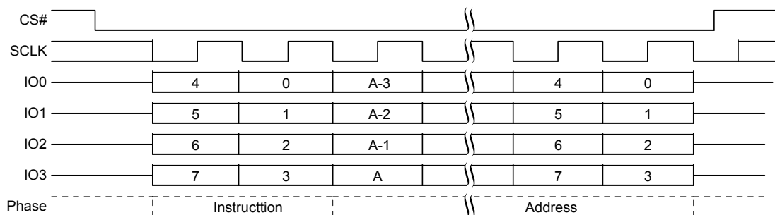
Figure 8.55 Sector Erase (SE 20h or 4SE 21h) QPI Mode Command Sequence
