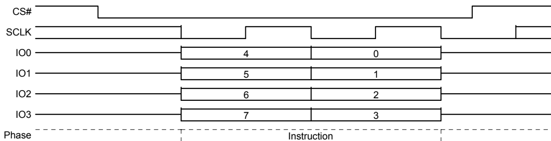
Figure 8.38 Exit QPI (QPIEX F5h) Command Sequence
