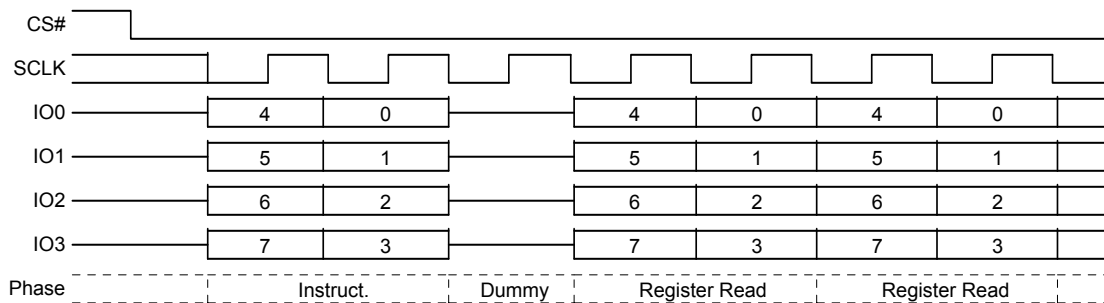
Figure 8.28 DLP Read (DLPRD) Command Sequence – QPI Mode
