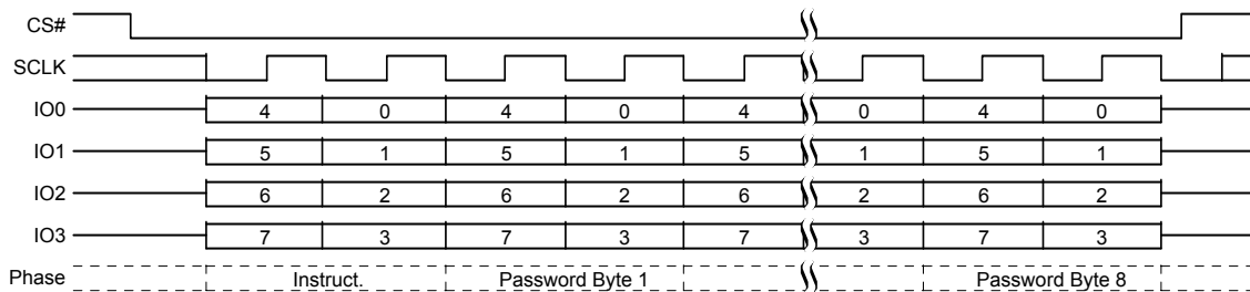
Figure 8.92 Password Program (PASSP) Command Sequence QPI mode
