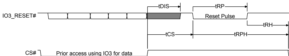
Figure 12.9 Hardware Reset when Quad or QPI Mode and IO3 / RESET# are Enabled
