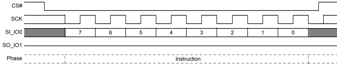
Figure 8.62 Program or Erase Suspend Command Sequence
