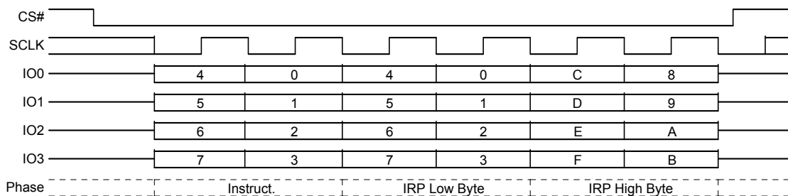
Figure 8.84 IRP Program (IRPP) Command QPI
