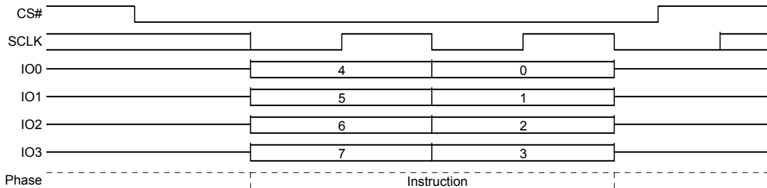
Figure 8.20 Write Enable for Volatile Registers (WRENV) Command Sequence QPI Mode
