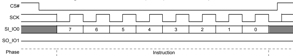
Figure 8.17 Write Disable (WRDI) Command Sequence
