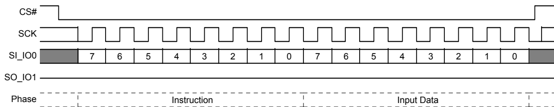
Figure 8.25 Write DLRV (WDLRV) Command Sequence
