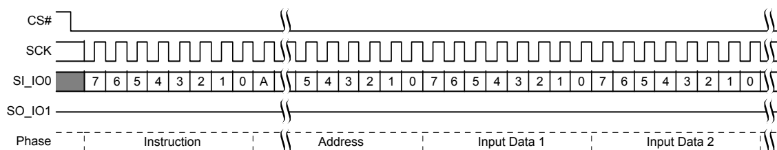
Figure 8.51 Page Program (PP 02h or 4PP 12h) Command Sequence
