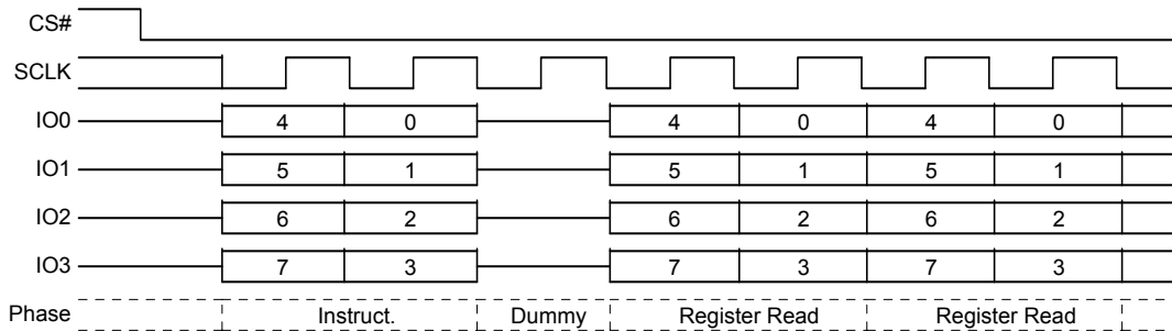
Figure 8.86 Protection Register Read (PRRD) Command Sequence – QPI Mode
