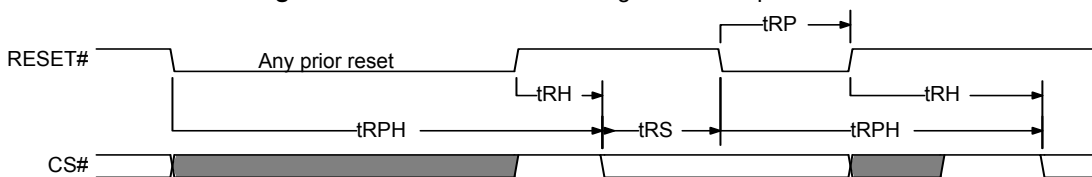
Figure 12.7 Hardware Reset using RESET# Input
