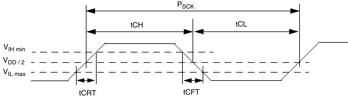
Figure 12.10 Clock Timing
