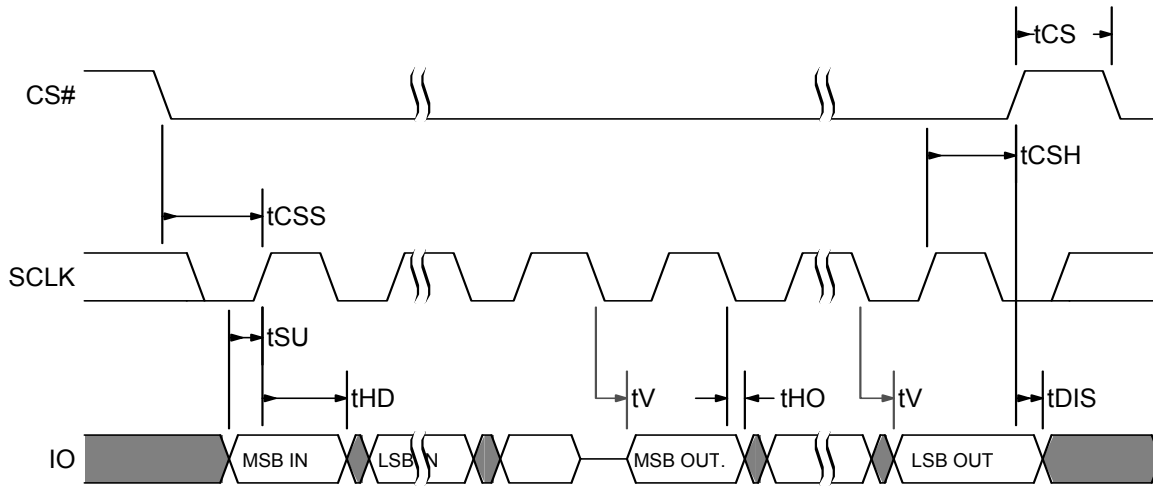
Figure 12.13 SDR MIO Timing
