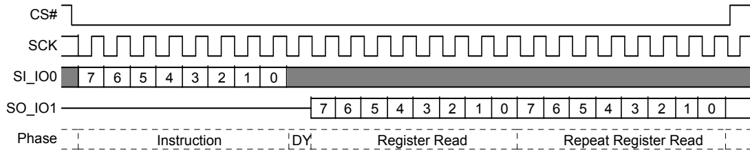
Figure 8.27 DLP Read (DLPRD) Command Sequence
