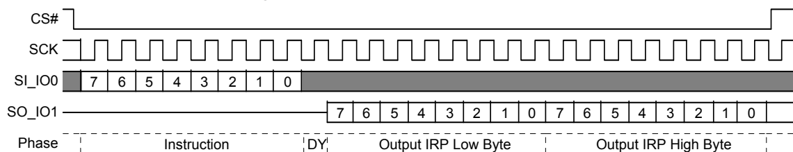
Figure 8.81 IRPRD Command Sequence
