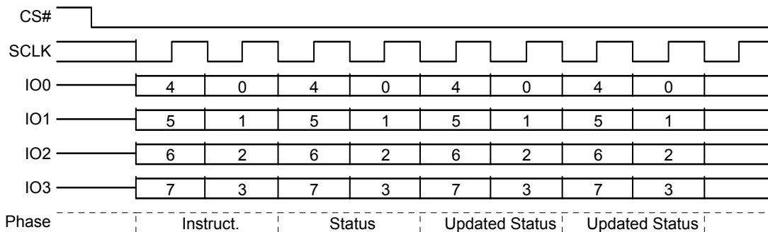
Figure 8.10 Read Status Register 1 (RDSR1) QPI Mode Command
