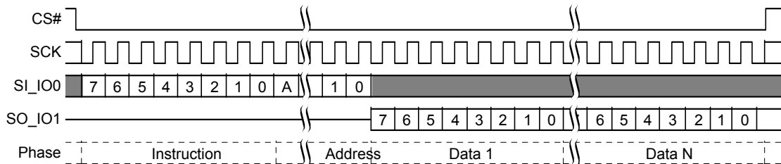
Figure 8.39 Read Command Sequence
