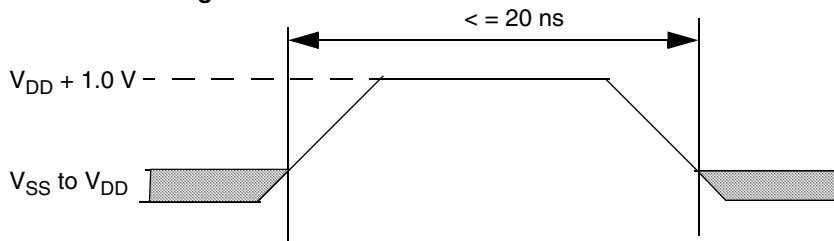
Figure 11.2 Maximum Positive Overshoot Waveform
