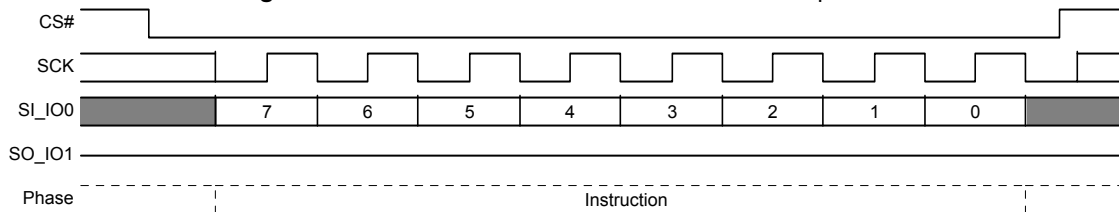
Figure 8.95 Software / Mode Bit Reset Command Sequence
