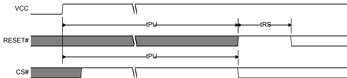
Figure 12.6 POR followed by Hardware Reset
