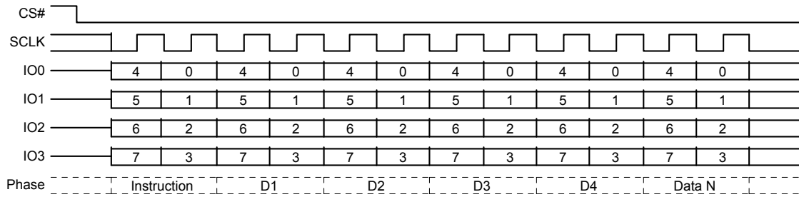
Figure 8.3 Read Quad Identification (RDQID) Command Sequence QPI Mode
