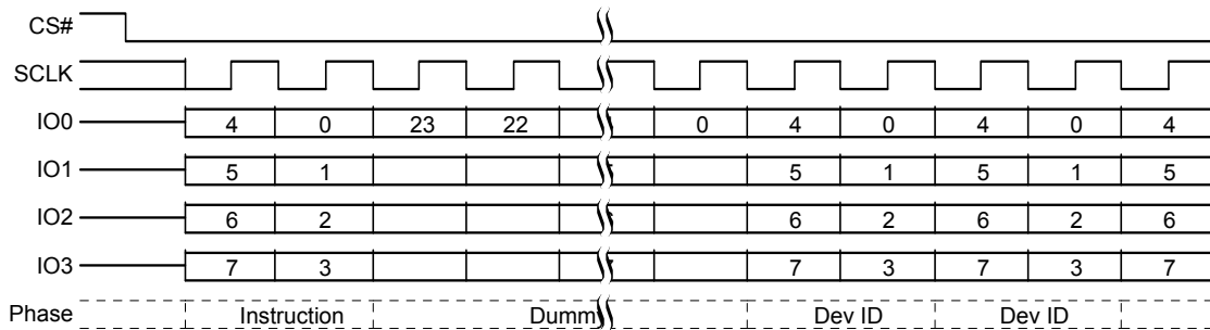
Figure 8.102 Read Identification (RES) QPI Mode Command
