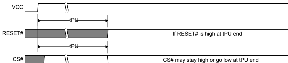
Figure 12.5 Reset high at the end of POR
