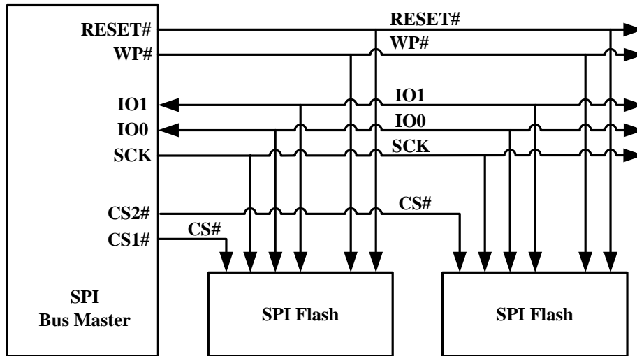
Figure 4.2 Bus Master and Memory Devices on the SPI Bus - Dual Bit Data Path
