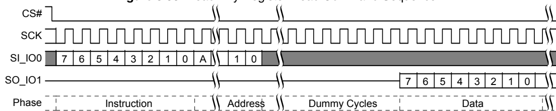
Figure 8.33 Read Any Register Read Command Sequence
