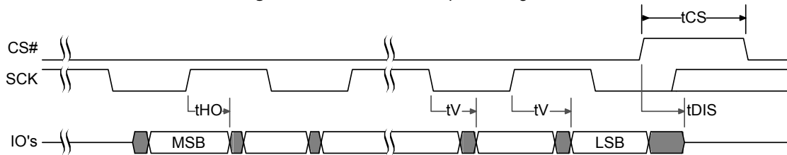
Figure 12.16 SPI DDR Output Timing
