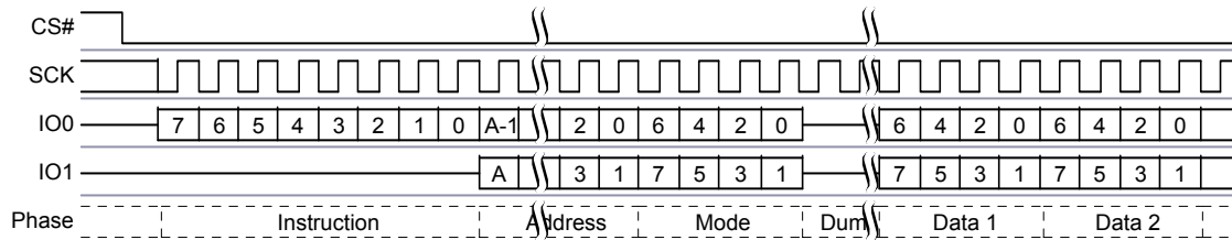
Figure 8.43 Dual I/O Read Command Sequence
