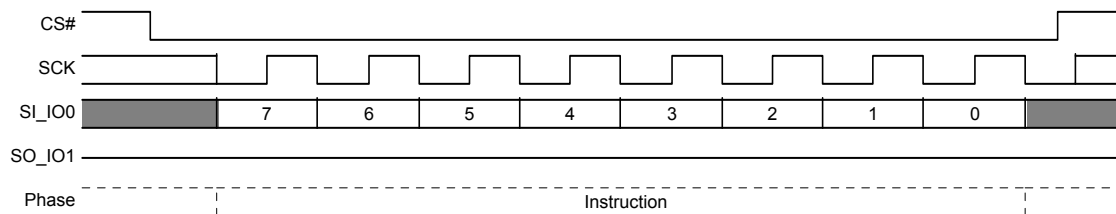
Figure 8.87 Protection Register Lock (PRL) Command Sequence
