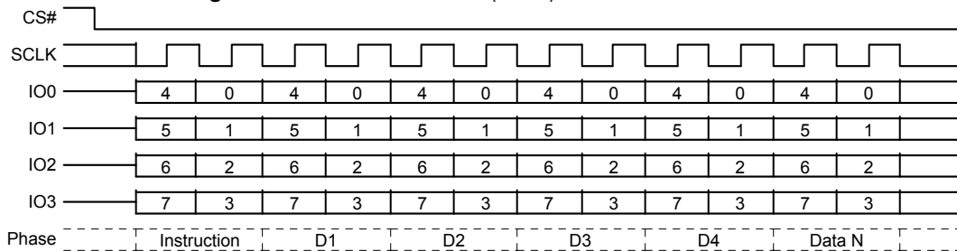
Figure 8.2 Read Identification (RDID) QPI Mode Command
