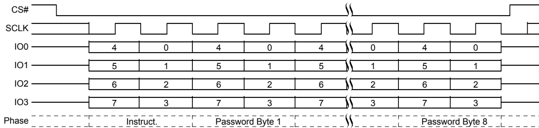
Figure 8.94 Password Unlock (PASSU) Command Sequence QPI mode
