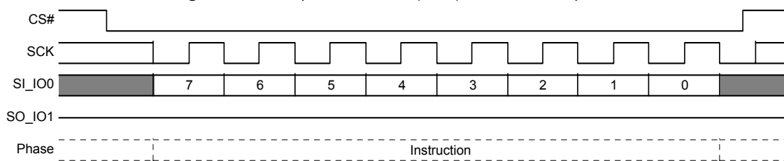
Figure 8.97 Deep Power Down (DPD) Command Sequence
