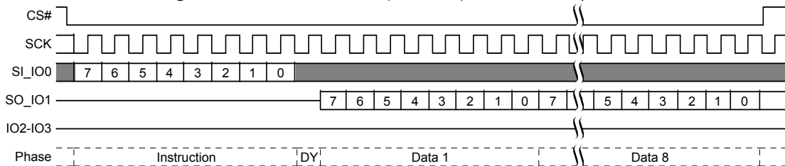
Figure 8.89 Password Read (PASSRD) Command Sequence
