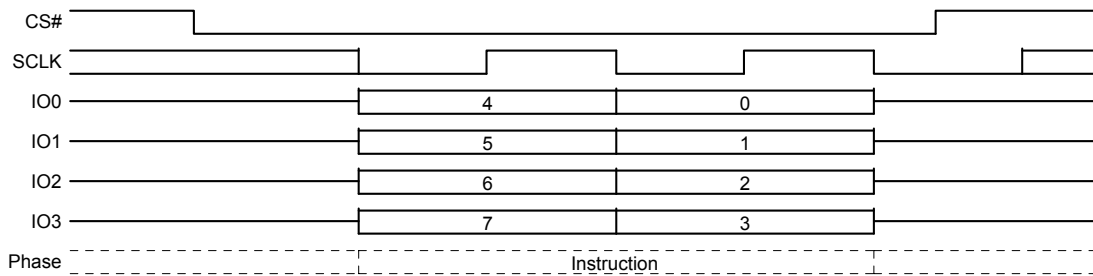
Figure 8.98 Deep Power Down (DPD) Command Sequence – QPI Mode
