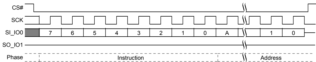
Figure 8.58 Block Erase (BE D8h or 4BE DCh) Command Sequence
