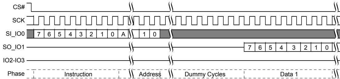
Figure 8.40 Fast Read (FAST_READ) Command Sequence
