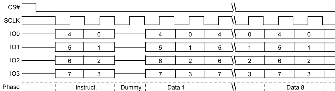
Figure 8.90 Password Read (PASSRD) Command Sequence – QPI Mode
