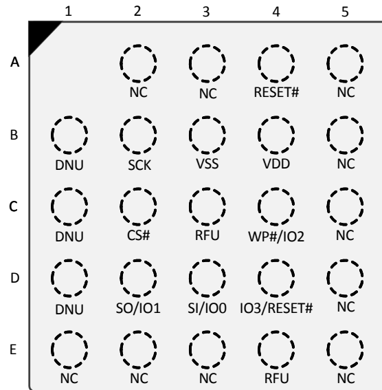
Figure 2.3 24-Ball BGA, 5x5 Ball Footprint (FAB024), Top View
