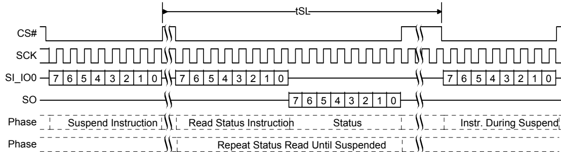
Figure 8.64 Program or Erase Suspend Command with Continuing Instruction Commands Sequence
