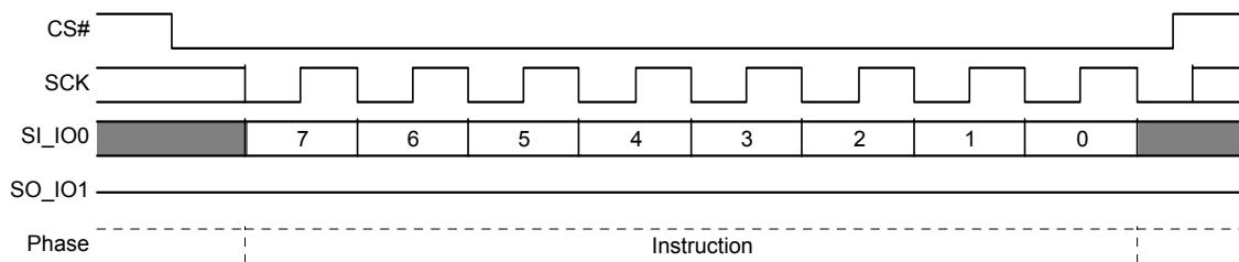
Figure 8.99 Release from Deep Power Down (RES) Command Sequence
