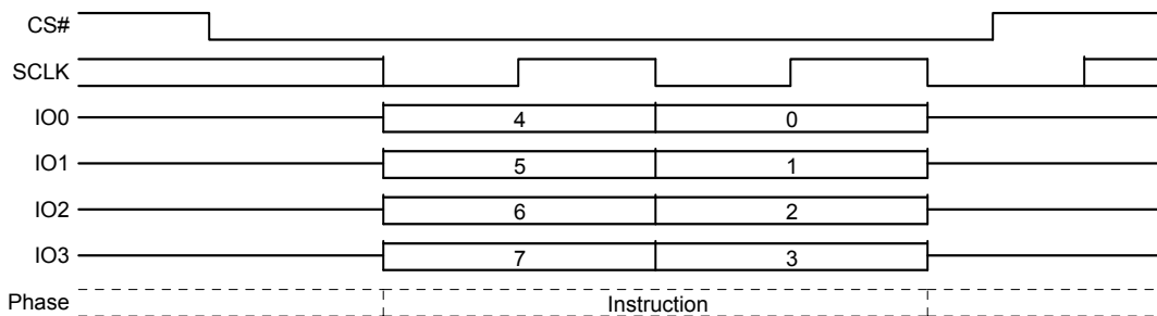
Figure 8.96 Software Reset / Mode Bit Command Sequence – QPI Mode
