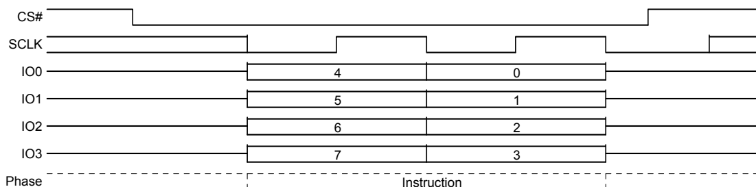
Figure 8.100 Release from Deep Power Down (RES) Command Sequence – QPI Mode
