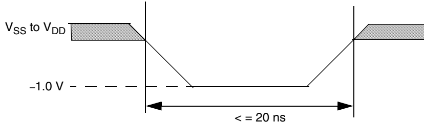
Figure 11.1 Maximum Negative Overshoot Waveform
