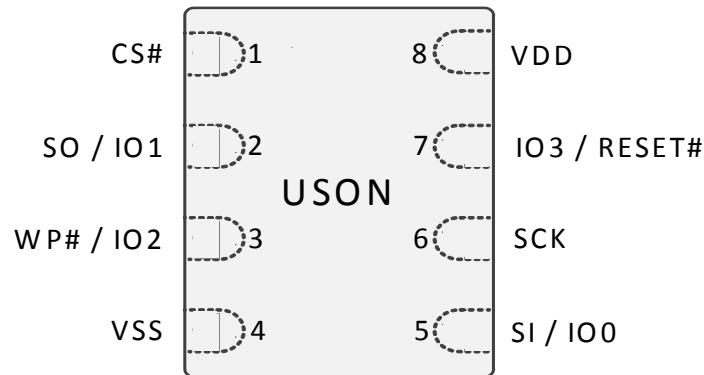
Figure 2.2 8-Connector Package (USON 4x4), Top View
