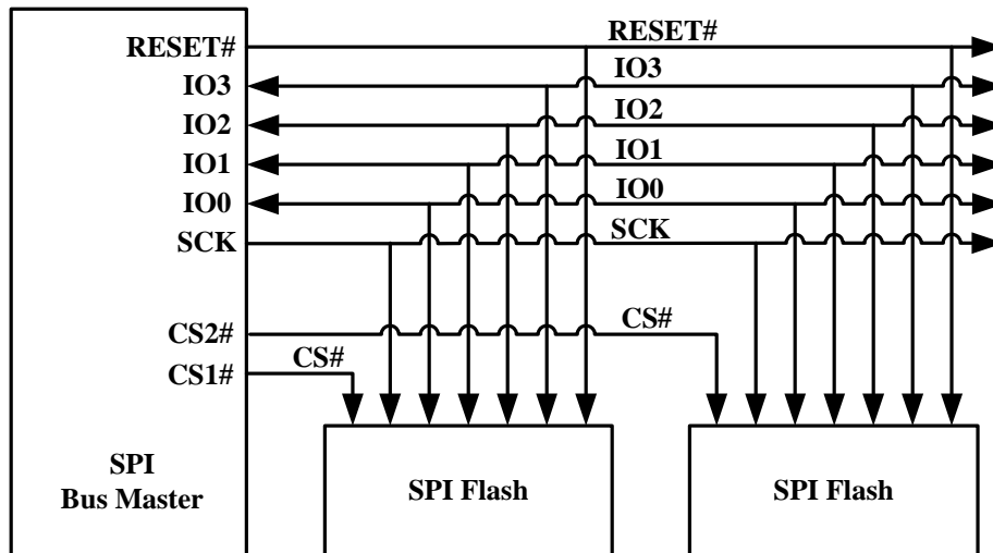
Figure 4.3 Bus Master and Memory Devices on the SPI Bus - Quad Bit Data Path - Separate RESET#
