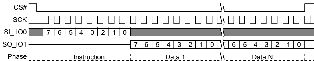
Figure 8.1 Read Identification (RDID) Command Sequence
