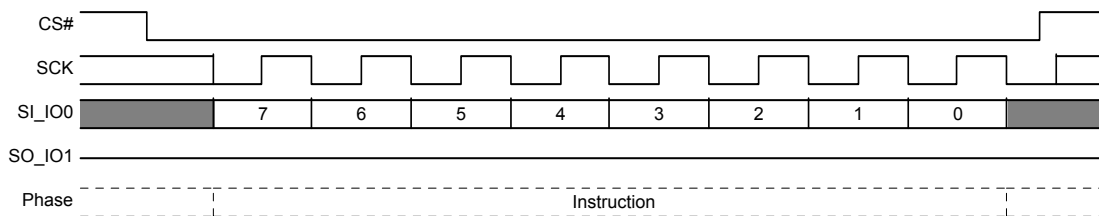
Figure 8.37 Enter QPI Mode (QPIEN 38h) Command Sequence
