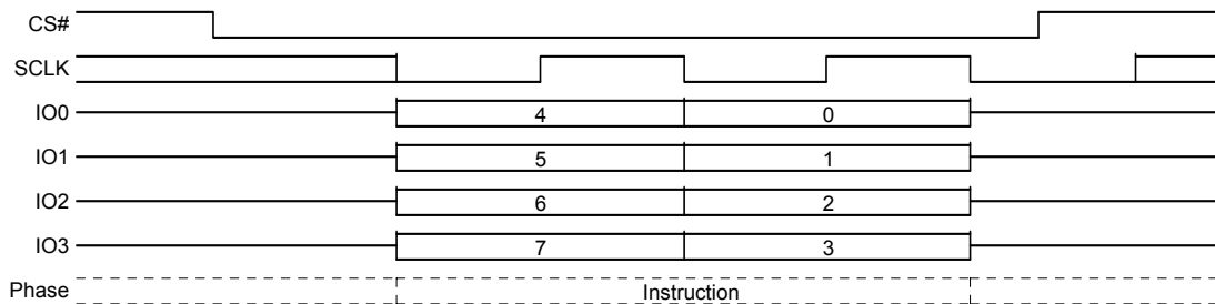
Figure 8.76 Global IBL Lock (GBL) Command Sequence QPI mode
