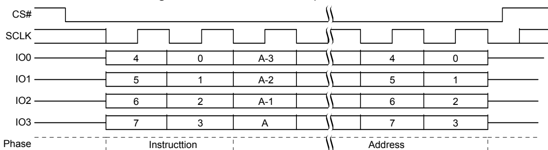
Figure 8.72 IBL Command Sequence QPI Mode
