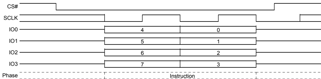
Figure 8.16 Write Enable (WREN) Command Sequence QPI Mode
