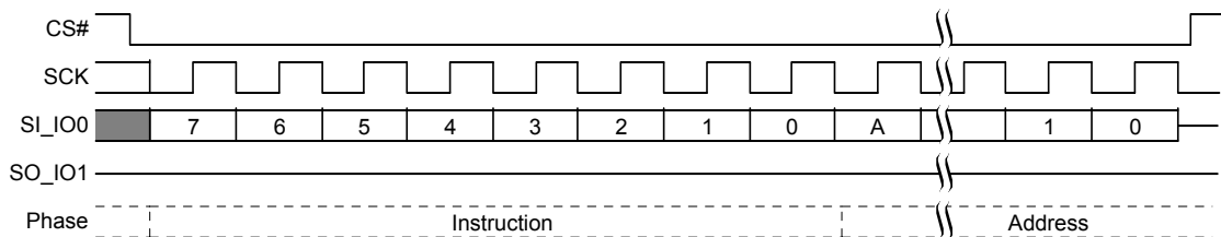
Figure 8.56 Half Block Erase (HBE 52h or 4HBE 53h) Command Sequence
