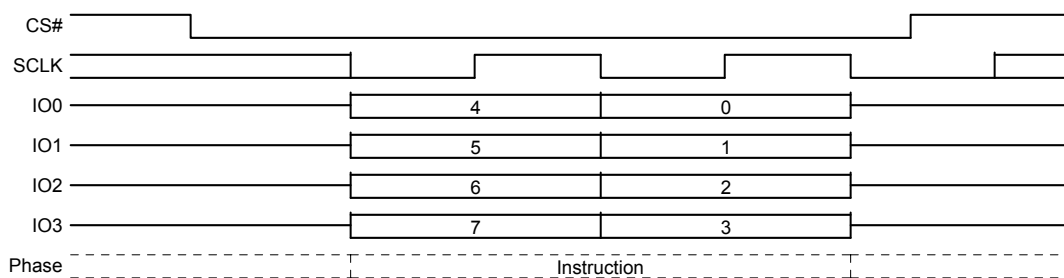
Figure 8.66 Erase or Program Resume command Sequence QPI mode
