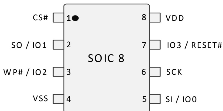
Figure 2.1 8-Pin Plastic Small Outline Package (SOIC8)
