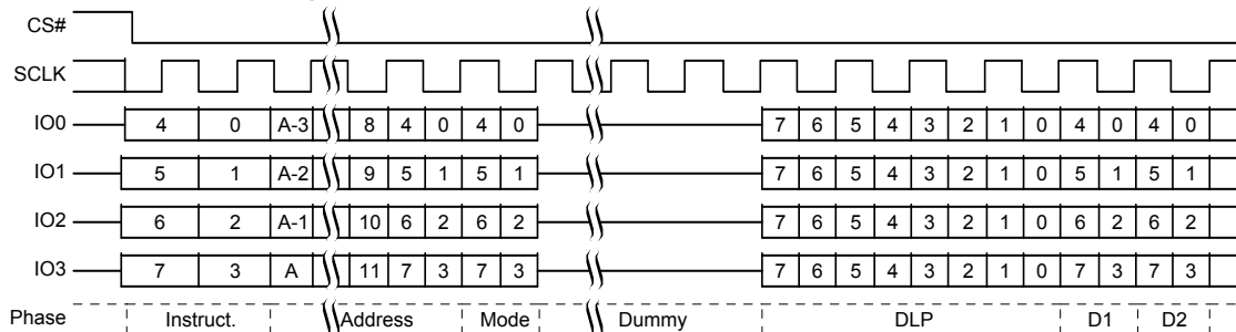
Figure 8.49 DDR Quad I/O Read Initial Access QPI Mode
