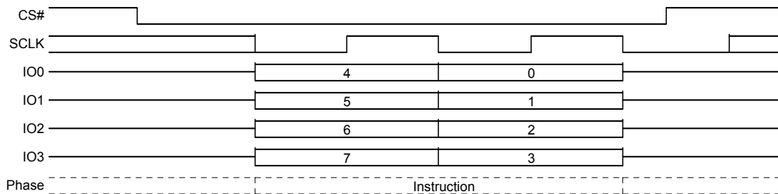
Figure 8.22 Clear Status Register (CLSR) QPI Mode
