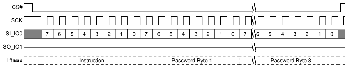
Figure 8.91 Password Program (PASSP) Command Sequence
