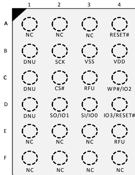
Figure 2.4 24-Ball BGA, 4x6 Ball Footprint (FAC024), Top View
