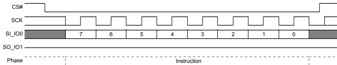
Figure 8.19 Write Enable for Volatile Registers (WRENV) Command Sequence
