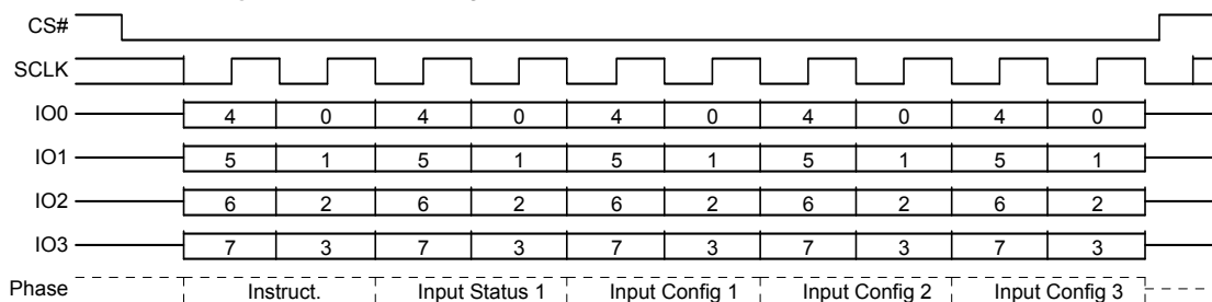
Figure 8.14 Write Register (WRR) Command Sequence QPI Mode
