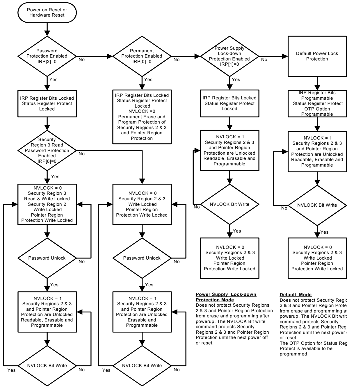
Figure 7.3 Permanent, Password and Power Supply Lock-down Protection Overview
