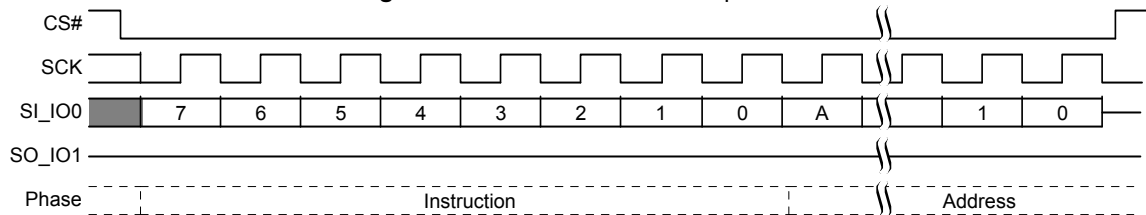
Figure 8.79 SPRP Command Sequence
