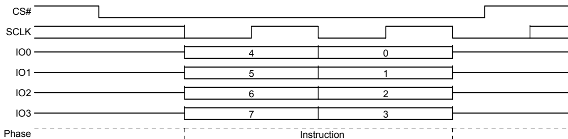
Figure 8.78 Global IBL Unlock (GBUL) Command Sequence QPI mode
