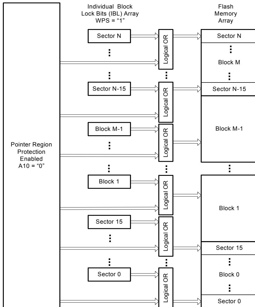
Figure 7.2 Individual Block Lock / Pointer Region Protection Control
