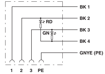
Contact assignment of valve connector
