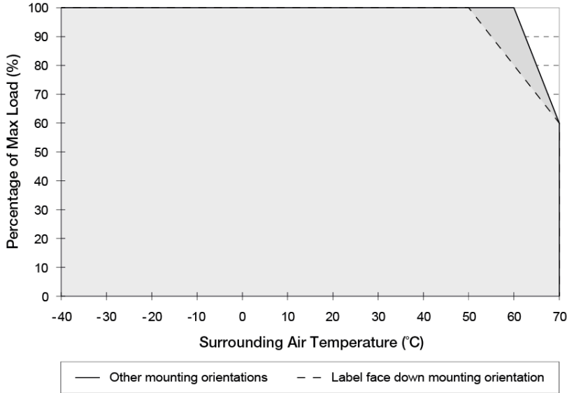
Fig. 1 De-rating for Label face down mounting orientation
