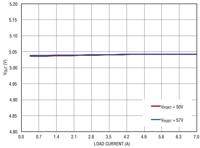
Figure 3. Output Voltage Regulation
