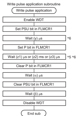
Note 7: Write Pulse Width
