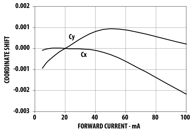
Figure 7. Chromaticity Shift Vs. forward current
