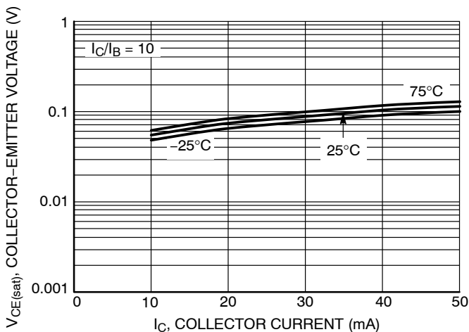
Figure 51. V_{CE(sat)} vs. I_C
