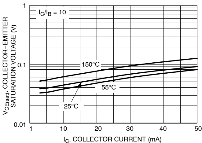
Figure 56. V_{CE(sat)} versus I_C
