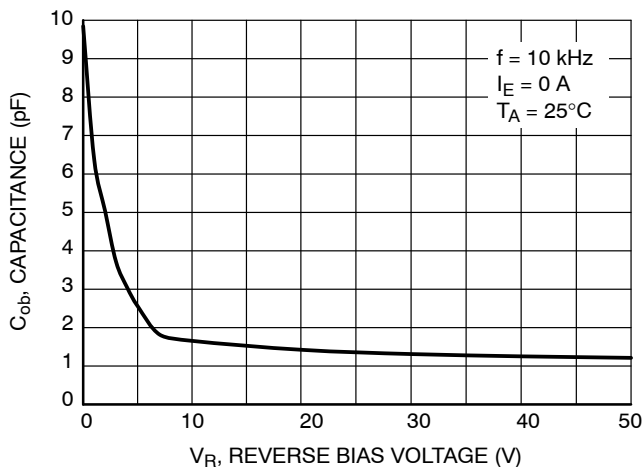
Figure 53. Output Capacitance
