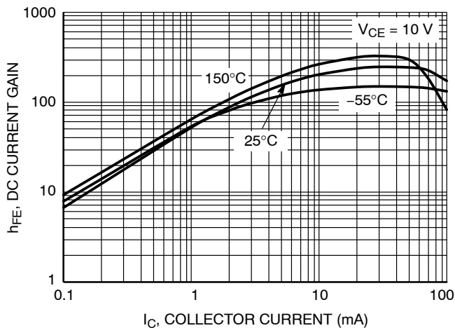
Figure 57. DC Current Gain
