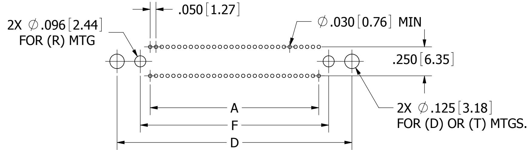
PCB LAYOUT, CONNECTOR SIDE
