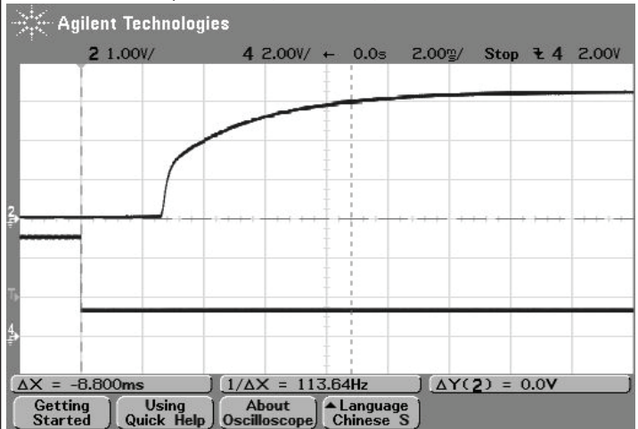
On/Off Enable Delay (Vin=48V, Vout=nom., Iout=30A, Cloud=10 \mu F, Ta=+25° C., ScopeBW=20Mhz, Trace 2=Vout, Trace 4=Enable).
