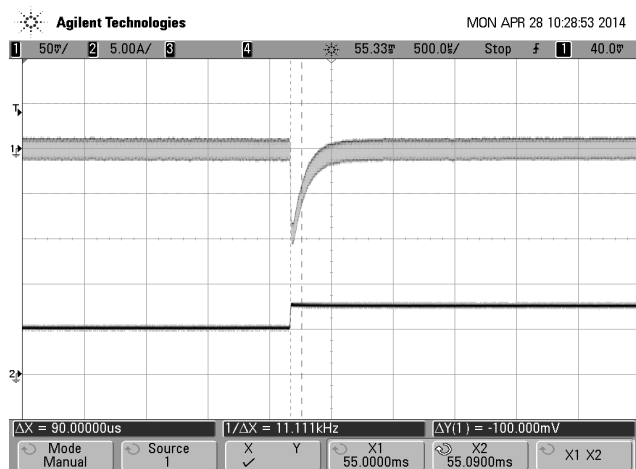
Step Load Transient Response (Vin=48V, Vout=nom., Cload=220uF, Iout=50% to 75% of full load, Ta=25° C) Trace 1=Vout, 50mV/div., 500µS/div.
