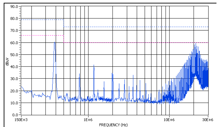
Graph 7. Conducted emissions performance, Positive Line, CISPR 22, Class A, full load
