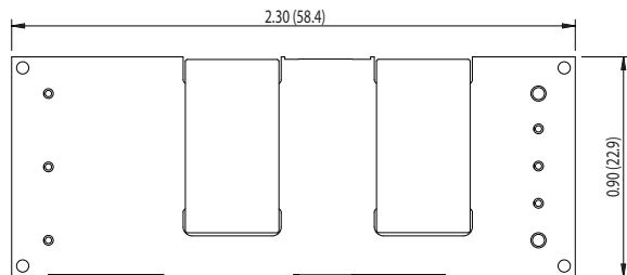
OPEN FRAME (NO BASEPLATE)
