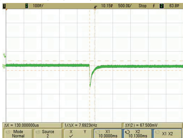
Step Load Transient Response (Slew=1A / \mu Sec., Vin=48V., Clod=0, Iout=22.5A to 15A)
