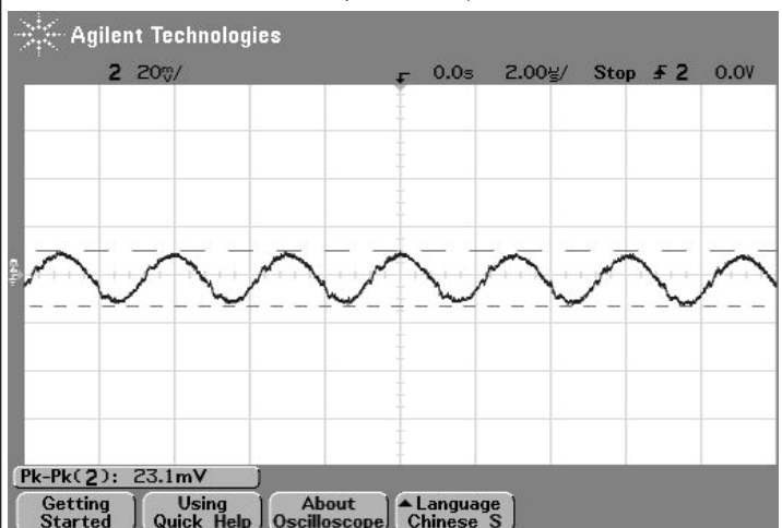
Output Ripple and noise (Vin=48V, Vout=nom., Iout=30A, Cloud=0, Ta=+25° C., ScopeBW=20Mhz)
