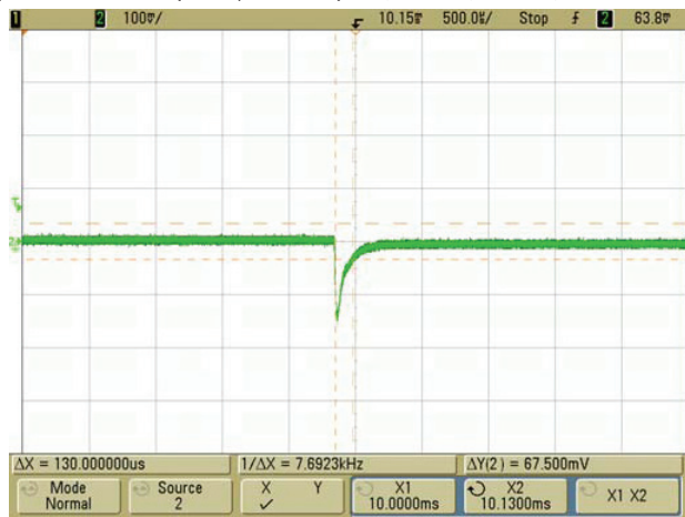
Step Load Transient Response (Slew=1A / \mu Sec., Vin=48V., Cloud=0, Iout=22.5A to 15A)
