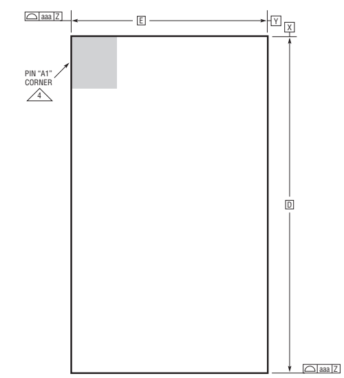
PACKAGE TOP VIEW
