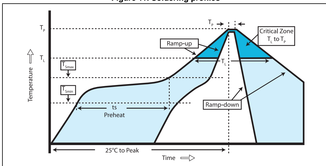
Figure 11. Soldering profiles
