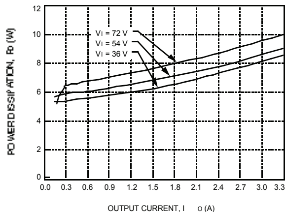
Figure 28. JW050C Power Dissipation vs. Output Current
