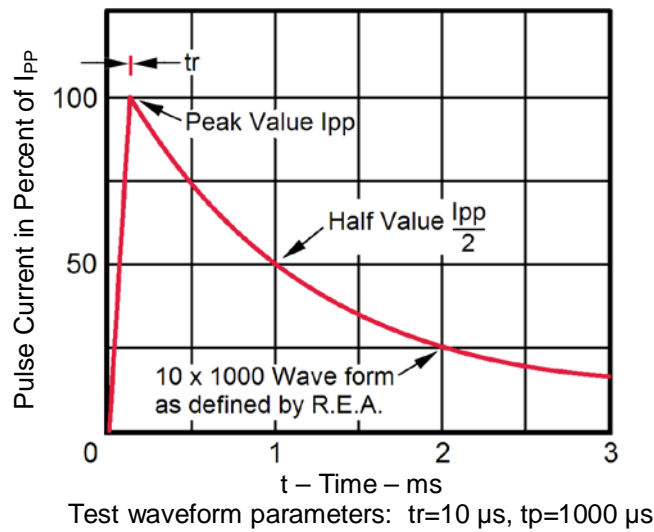
FIGURE 2 Pulse Waveform for 10/1000 μs Exponential Surge
