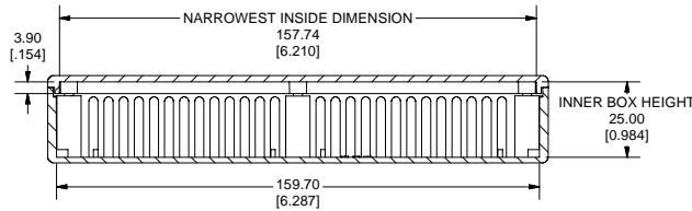
SECTION C-C
