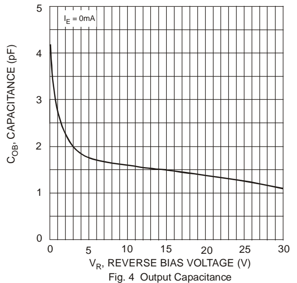
Fig. 4 Output Capacitance
