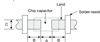
Land patterns for PCBs
