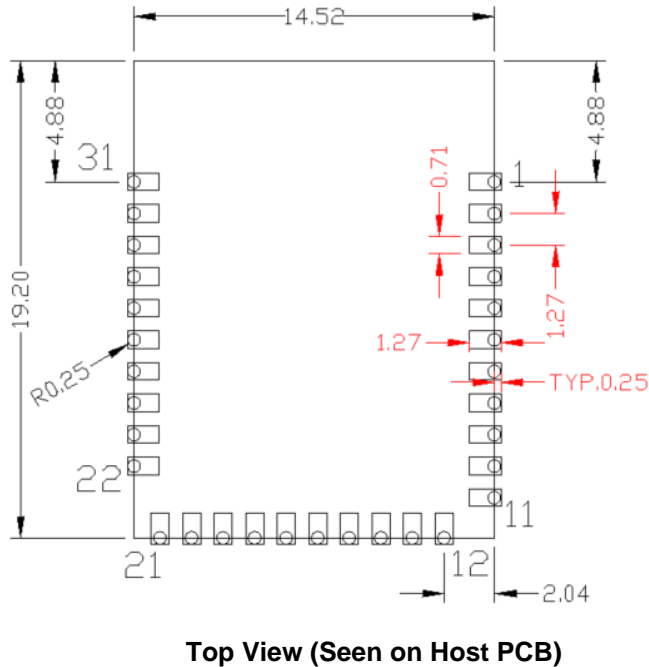
Figure 4. Host Layout Pattern for CYBLE-2120XX-X0
