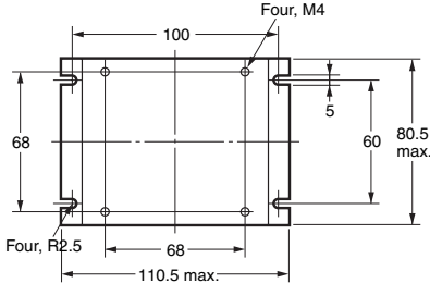
Mounting Holes
