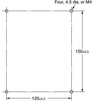
Mounting Holes
