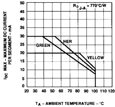
Figure 4. Maximum Allowable DC Current vs. Ambient Temperature.
