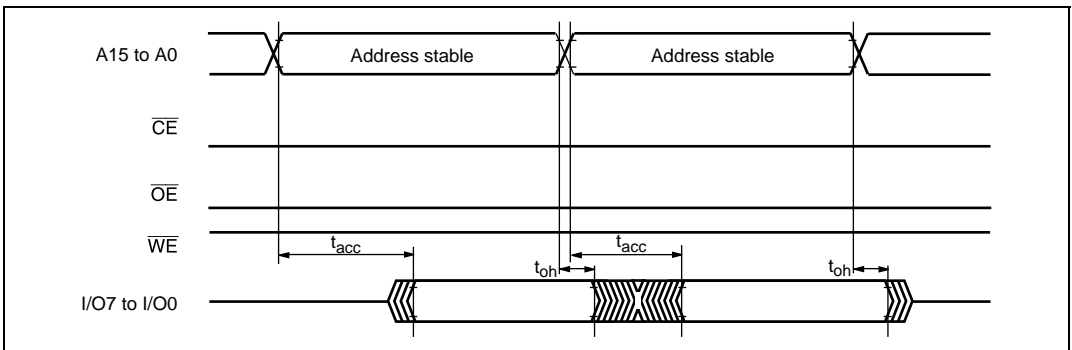
Figure 6.15 Timing Waveforms in \overline{\text{CE}} and \overline{\text{OE}} Enable State Read
