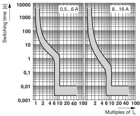
Trigger characteristic in the DC range
