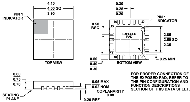
Figure 65. 20-Lead Lead Frame Chip Scale Package [LFCSP_WQ] 4 mm x 4 mm Body, Very Very Thin Quad (CP-20-10) Dimensions shown in millimeters
